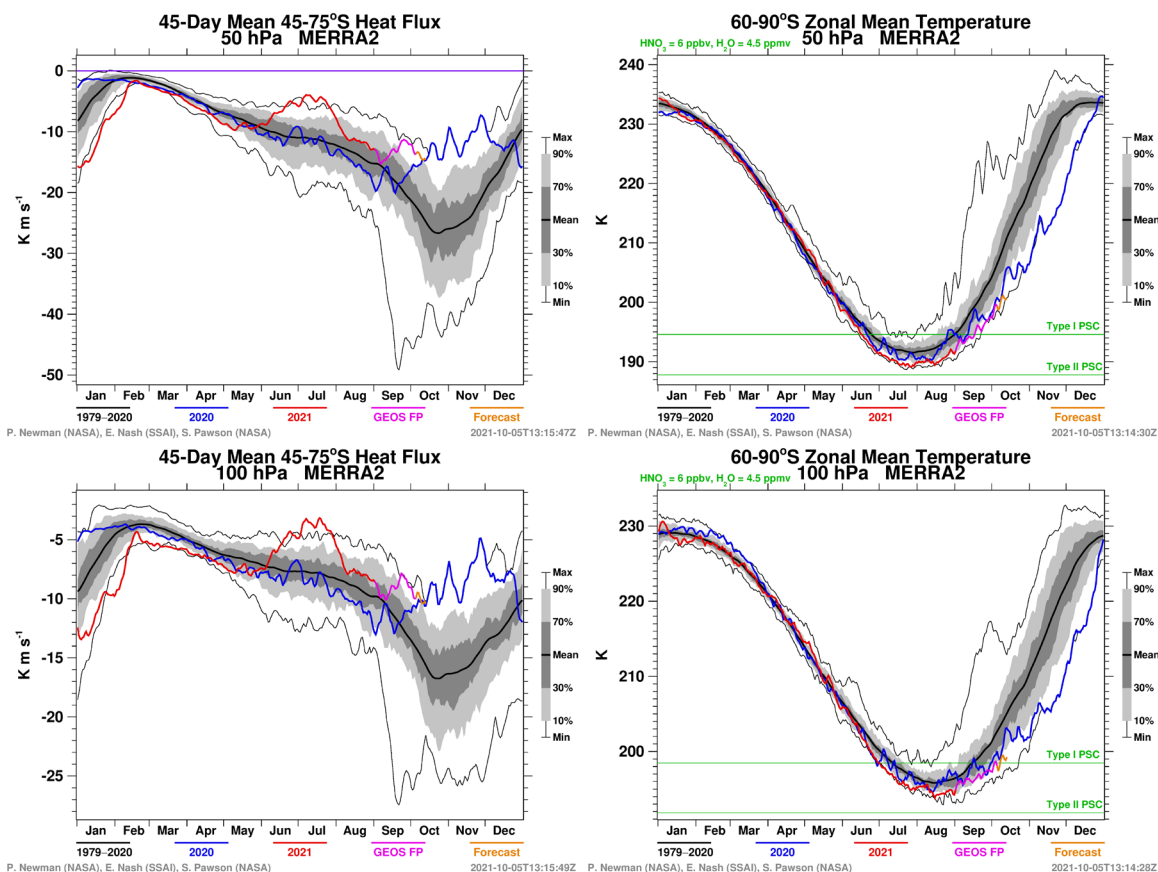
Figure 6 MERRA2 45-day mean 45°S-75°S eddy heat flux and 60°S-90°S zonal mean temperature at 50 & 100 hPa. Images courtesy of NASA GSFC, downloaded 6 October 2021, data through to 13 October 2021 (data starting 2021-09-01 are from GEOS FP; 2021-10-05 onwards are forecasts): http://ozonewatch.gsfc.nasa.gov/meteorology/SH.html
