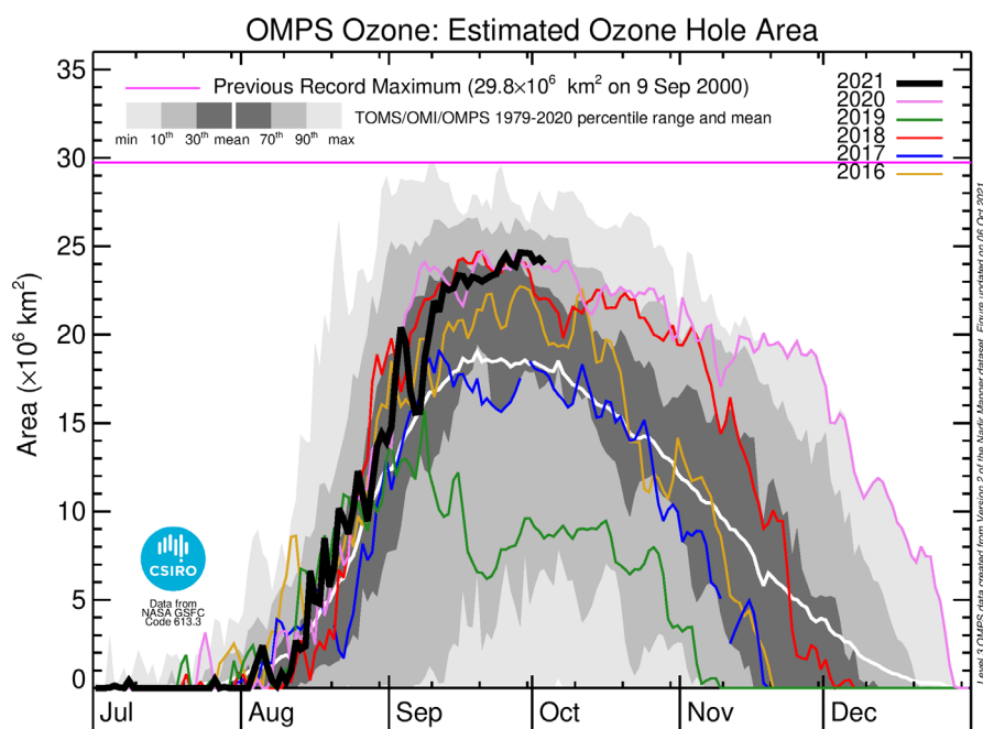
Figure 1 Ozone hole area based on OMPS satellite data (data up to 3 October 2021).
