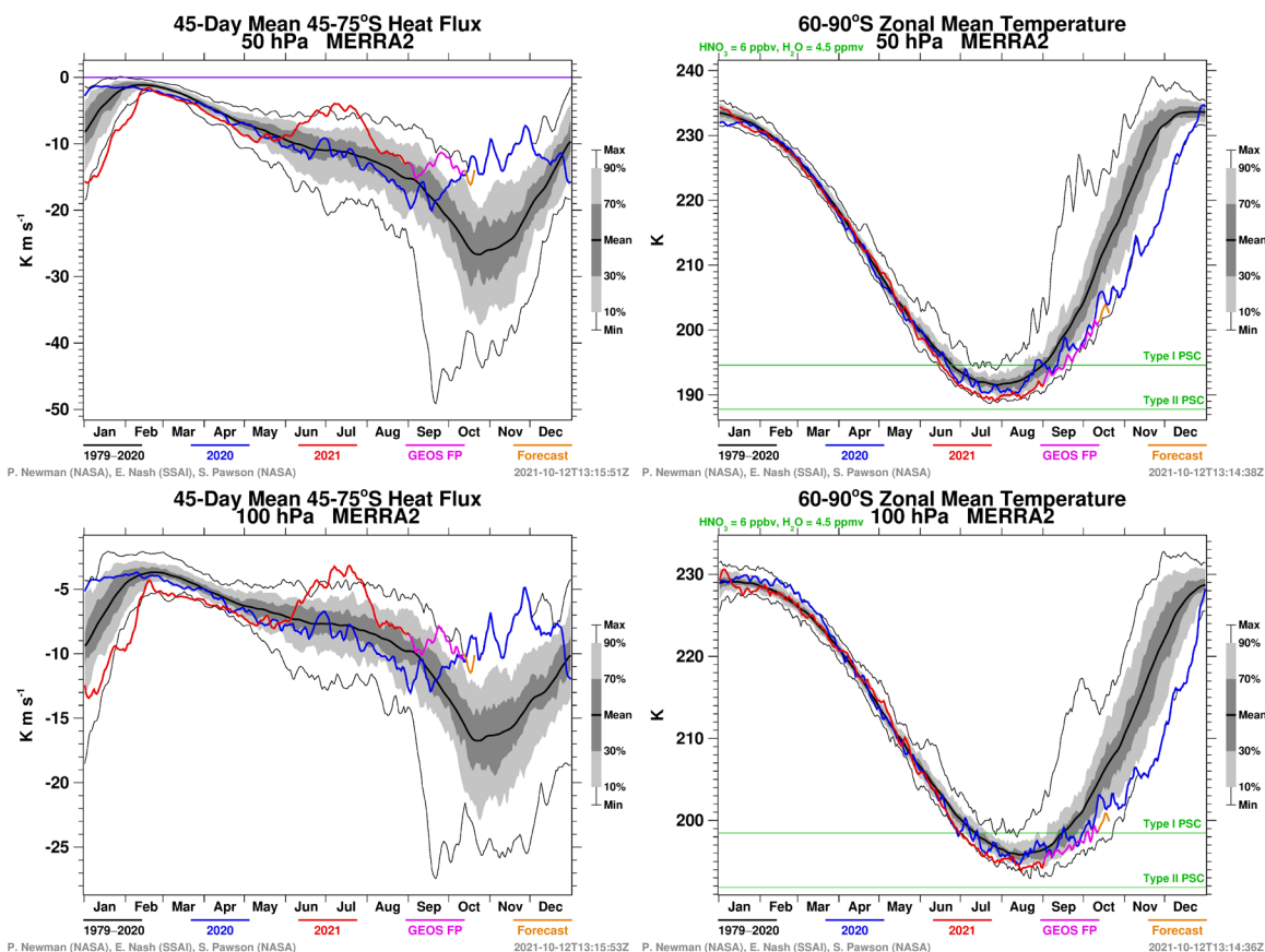
Figure 6 MERRA2 45-day mean 45°S-75°S eddy heat flux and 60°S-90°S zonal mean temperature at 50 & 100 hPa. Images courtesy of NASA GSFC, downloaded 13 October 2021, data through to 20 October 2021 (data starting 2021-09-01 are from GEOS FP; 2021-10-12 onwards are forecasts): http://ozonewatch.gsfc.nasa.gov/meteorology/SH.html
