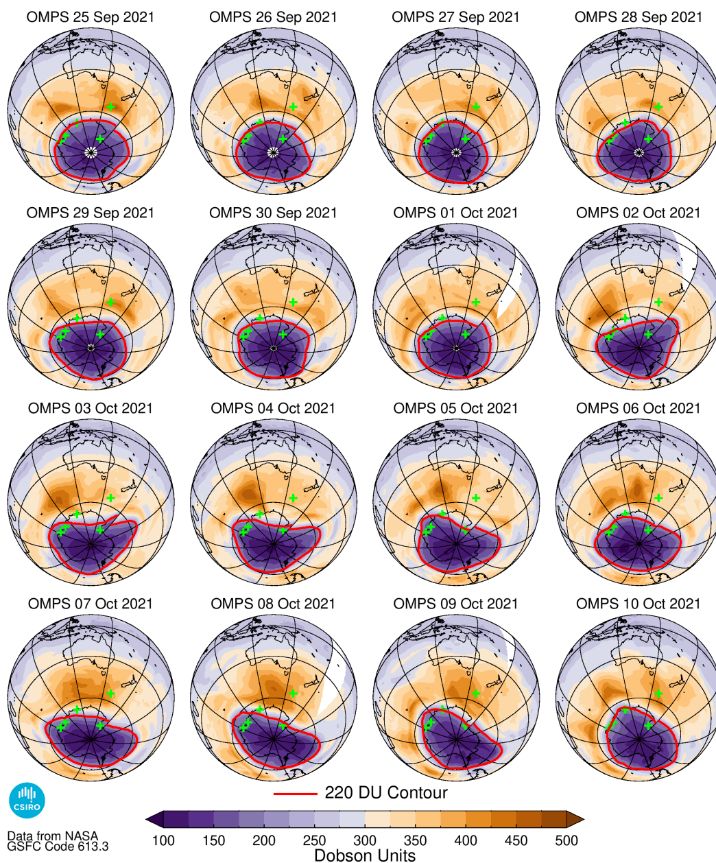
Figure 5 OMPS ozone hole images for 25 September – 10 October; the ozone hole boundary is indicated by the red 220 DU contour line. Green plus symbols indicate the location of the Australian Antarctic stations of Mawson (62.9°E, 67.6°S), Davis (78.0°E, 68.6°S) and Casey (110.5°E, 66.3°S), the New Zealand Antarctic station of Arrival Heights (166.7°E, 77.8°S) and Macquarie Island station (158.9°E, 54.5°S). The white area over Antarctica is missing data and indicates the approximate extent of the polar night. The OMPS instrument requires solar radiation to the earth's surface in order to measure the column ozone abundance.
