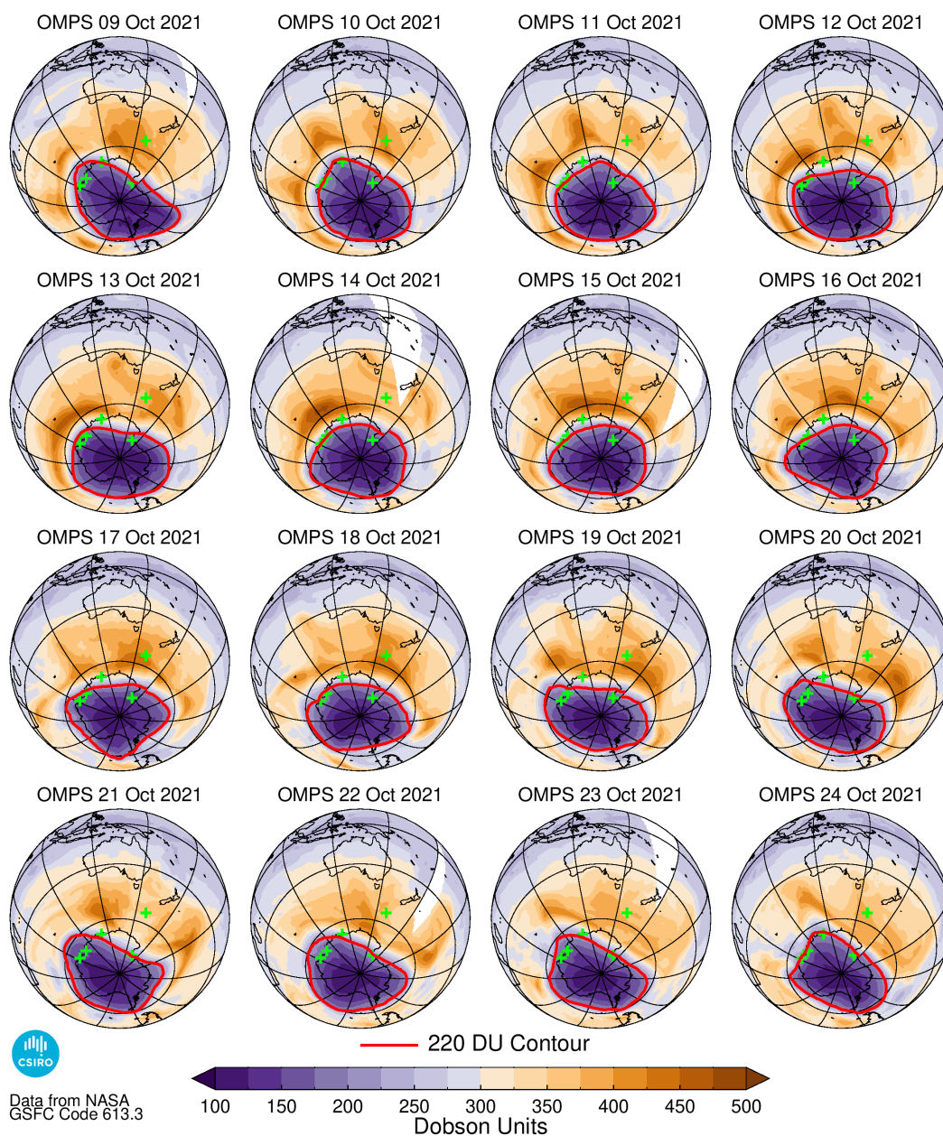
Figure 5 OMPS ozone hole images for 9 – 24 October; the ozone hole boundary is indicated by the red 220 DU contour line. Green plus symbols indicate the location of the Australian Antarctic stations of Mawson (62.9°E, 67.6°S), Davis (78.0°E, 68.6°S) and Casey (110.5°E, 66.3°S), the New Zealand Antarctic station of Arrival Heights (166.7°E, 77.8°S) and Macquarie Island station (158.9°E, 54.5°S).
