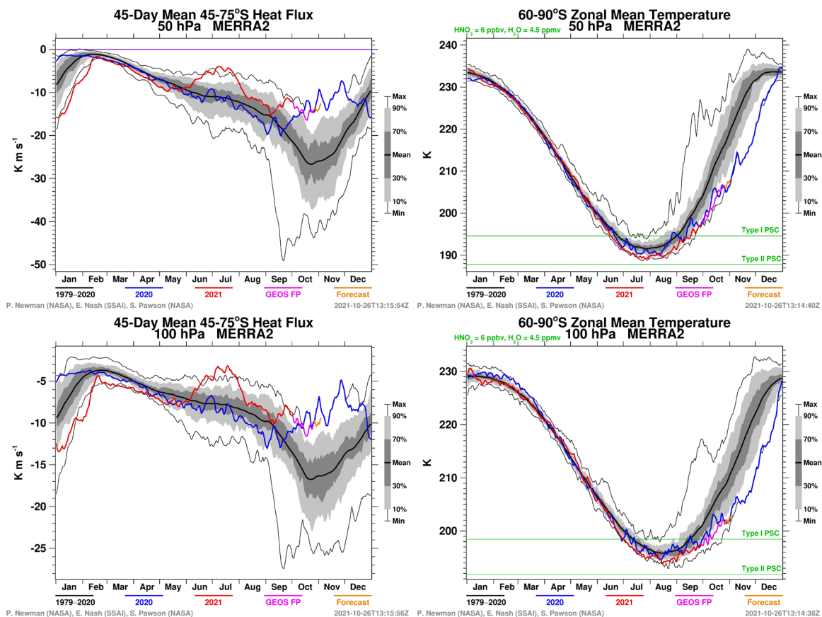
Figure 6 MERRA2 45-day mean 45°S-75°S eddy heat flux and 60°S-90°S zonal mean temperature at 50 & 100 hPa. Images courtesy of NASA GSFC, downloaded 27 October 2021, data through to 3 November 2021 (data starting 2021-10-01 are from GEOS FP; 2021-10-26 onwards are forecasts): http://ozonewatch.gsfc.nasa.gov/meteorology/SH.html
