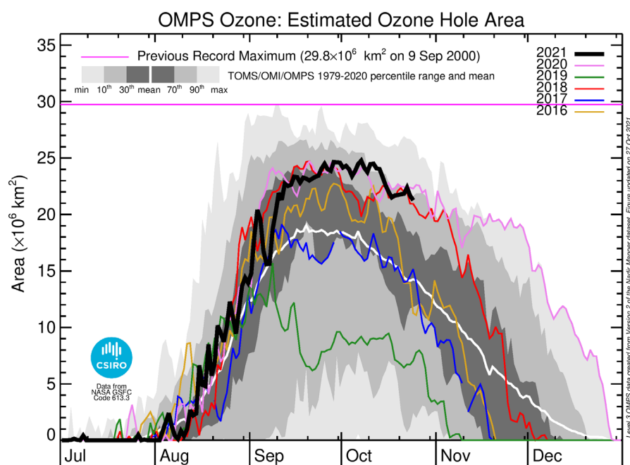
Figure 1 Ozone hole area based on OMPS satellite data (data up to 24 October 2021).
