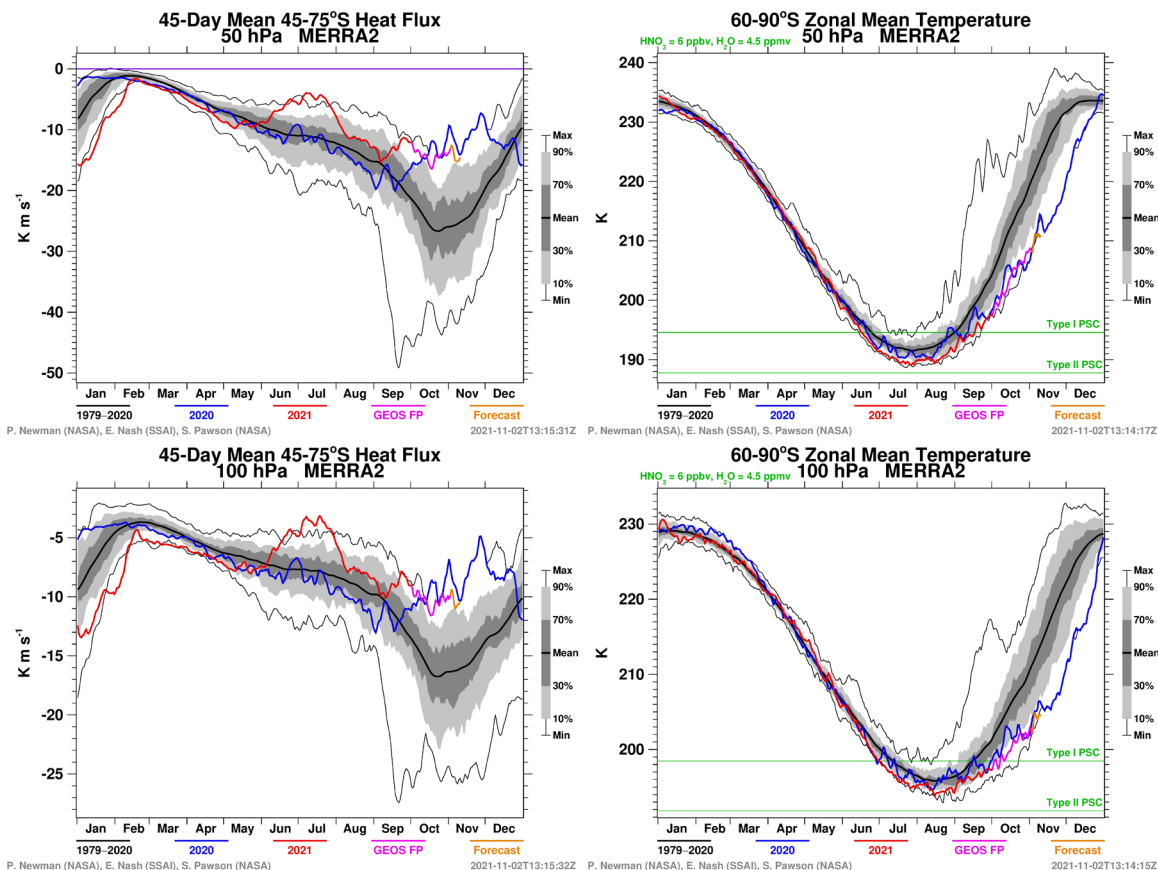
Figure 6 MERRA2 45-day mean 45°S-75°S eddy heat flux and 60°S-90°S zonal mean temperature at 50 & 100 hPa. Images courtesy of NASA GSFC, downloaded 3 November 2021, data through to 10 November 2021 (data starting 2021-10-01 are from GEOS FP; 2021-11-02 onwards are forecasts): http://ozonewatch.gsfc.nasa.gov/meteorology/SH.html
