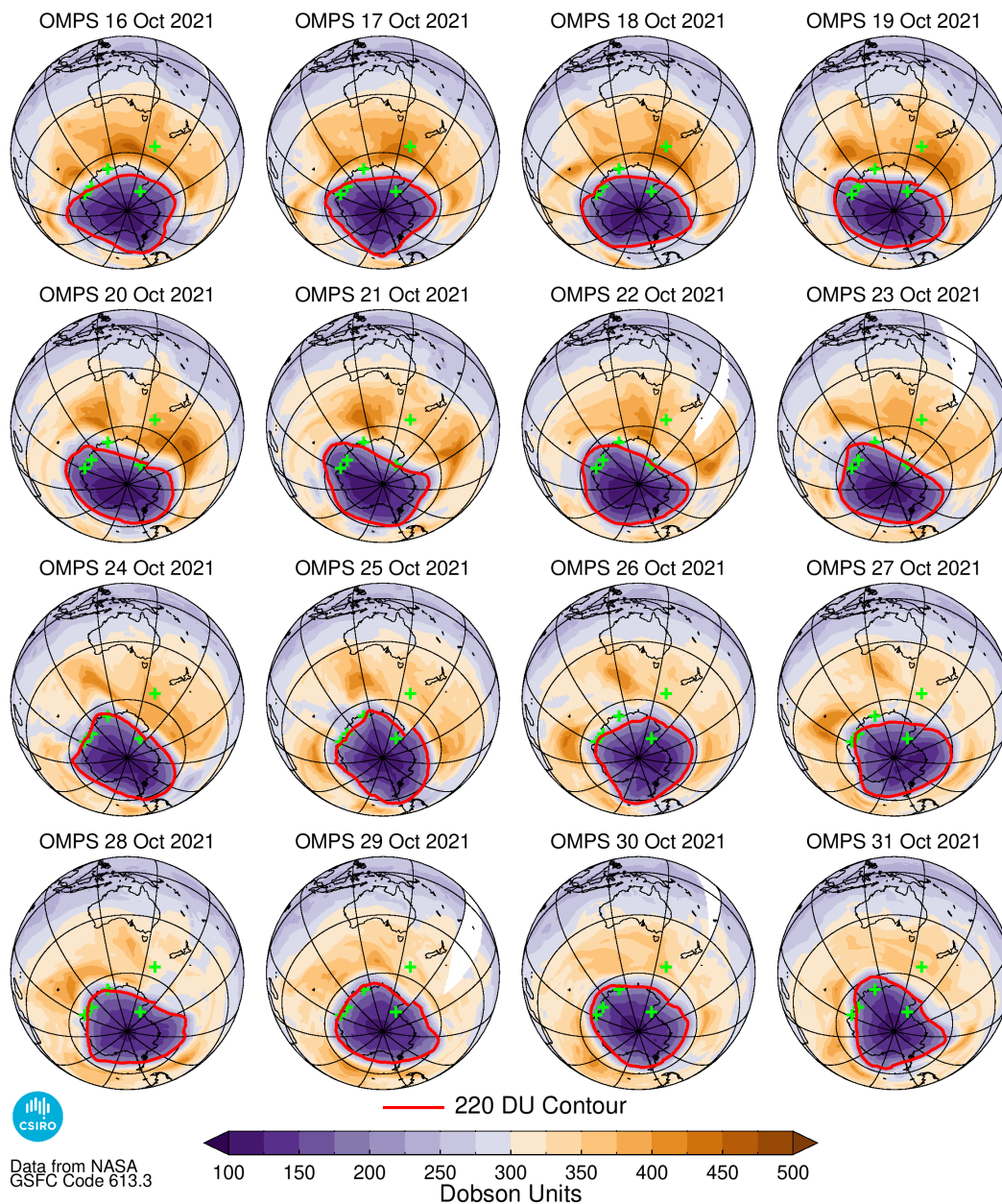
Figure 5 OMPS ozone hole images for 16 – 31 October; the ozone hole boundary is indicated by the red 220 DU contour line. Green plus symbols indicate the location of the Australian Antarctic stations of Mawson (62.9°E, 67.6°S), Davis (78.0°E, 68.6°S) and Casey (110.5°E, 66.3°S), the New Zealand Antarctic station of Arrival Heights (166.7°E, 77.8°S) and Macquarie Island station (158.9°E, 54.5°S).
