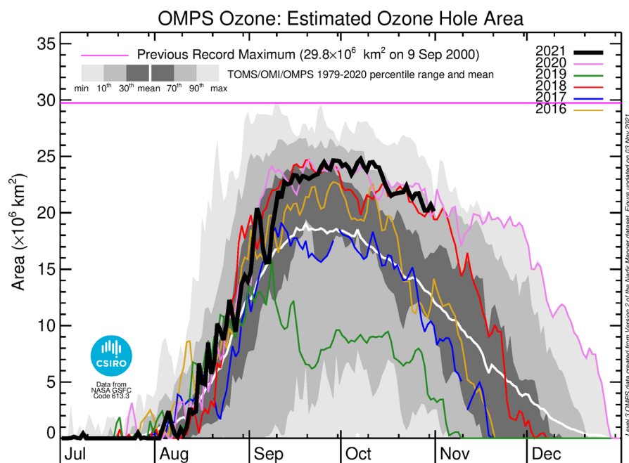
Figure 1 Ozone hole area based on OMPS satellite data (data up to 31 October 2021).
