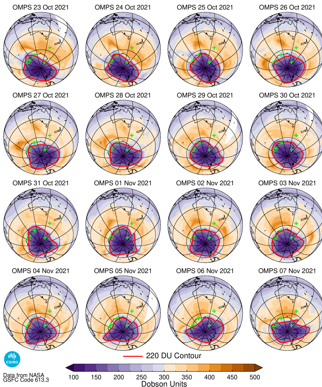
Figure 5 OMPS ozone hole images for 23 October – 7 November; the ozone hole boundary is indicated by the red 220 DU contour line. Green plus symbols indicate the location of the Australian Antarctic stations of Mawson (62.9°E, 67.6°S), Davis (78.0°E, 68.6°S) and Casey (110.5°E, 66.3°S), the New Zealand Antarctic station of Arrival Heights (166.7°E, 77.8°S) and Macquarie Island station (158.9°E, 54.5°S).
