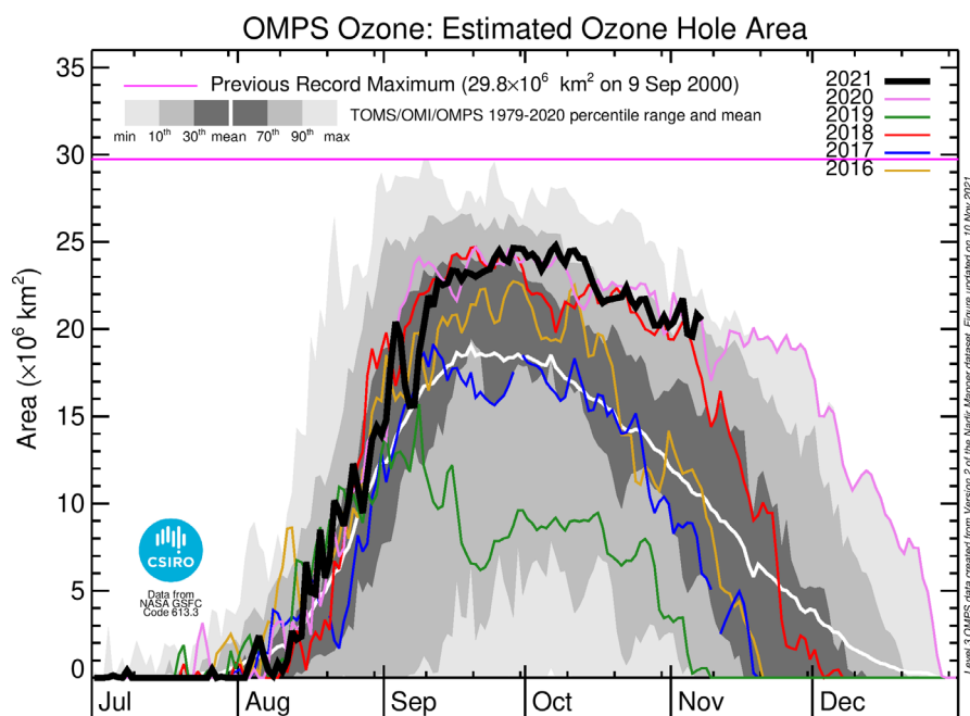
Figure 1 Ozone hole area based on OMPS satellite data (data up to 7 November 2021).
