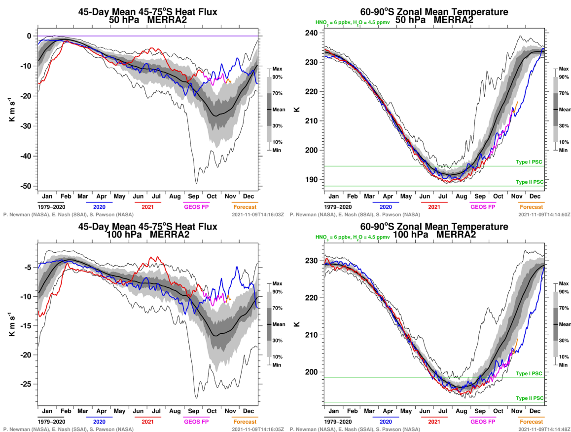
Figure 6 MERRA2 45-day mean 45°S-75°S eddy heat flux and 60°S-90°S zonal mean temperature at 50 & 100 hPa. Images courtesy of NASA GSFC, downloaded 10 November 2021, data through to 17 November 2021 (data starting 2021-10-01 are from GEOS FP; 2021-11-09 onwards are forecasts): http://ozonewatch.gsfc.nasa.gov/meteorology/SH.html
