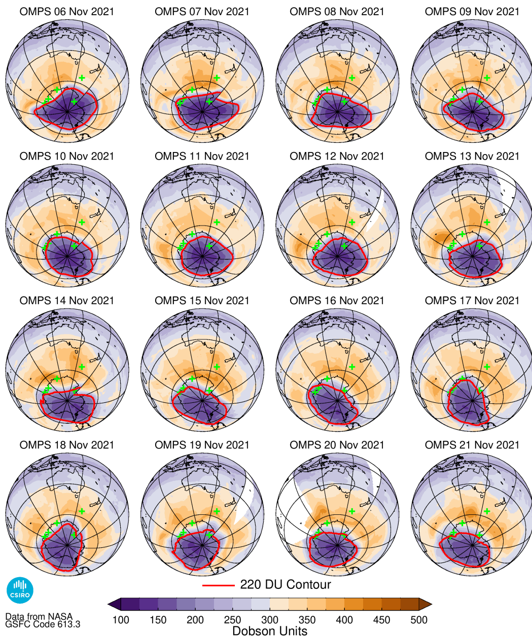
Figure 5 OMPS ozone hole images for 6 – 21 November; the ozone hole boundary is indicated by the red 220 DU contour line. Green plus symbols indicate the location of the Australian Antarctic stations of Mawson (62.9°E, 67.6°S), Davis (78.0°E, 68.6°S) and Casey (110.5°E, 66.3°S), the New Zealand Antarctic station of Arrival Heights (166.7°E, 77.8°S) and Macquarie Island station (158.9°E, 54.5°S).
