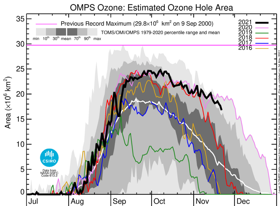
Figure 1 Ozone hole area based on OMPS satellite data (data up to 21 November 2021).
