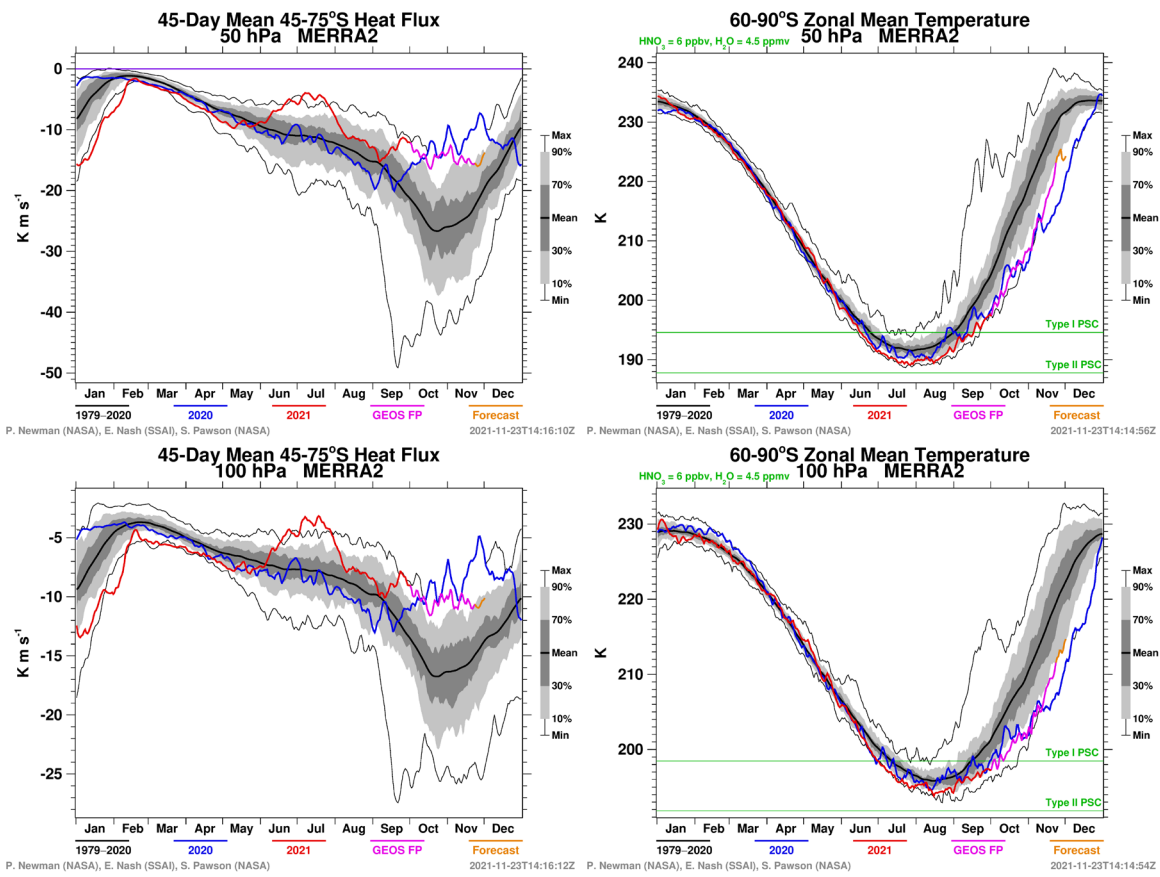
Figure 6 MERRA2 45-day mean 45°S-75°S eddy heat flux and 60°S-90°S zonal mean temperature at 50 & 100 hPa. Images courtesy of NASA GSFC, downloaded 24 November 2021, data through to 1 December 2021 (data starting 2021-10-01 are from GEOS FP; 2021-11-23 onwards are forecasts): http://ozonewatch.gsfc.nasa.gov/meteorology/SH.html
