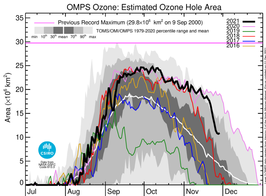
Figure 1 Ozone hole area based on OMPS satellite data (data up to 28 November 2021).
