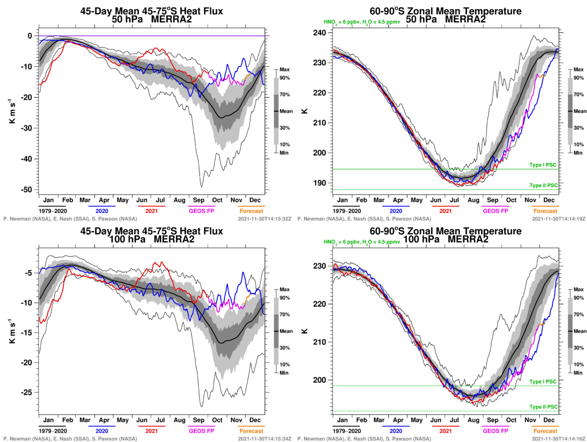
Figure 6 MERRA2 45-day mean 45°S-75°S eddy heat flux and 60°S-90°S zonal mean temperature at 50 & 100 hPa. Images courtesy of NASA GSFC, downloaded 1 December 2021, data through to 8 December 2021 (data starting 2021-10-01 are from GEOS FP; 2021-11-30 onwards are forecasts): http://ozonewatch.gsfc.nasa.gov/meteorology/SH.html
