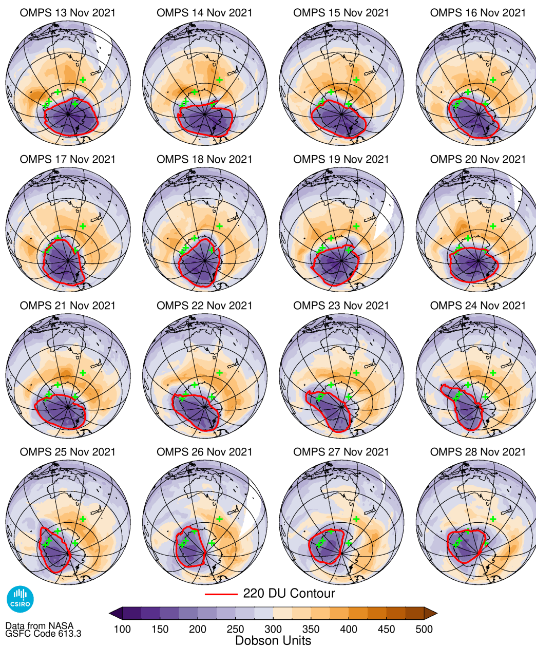
Figure 5 OMPS ozone hole images for 13 – 28 November; the ozone hole boundary is indicated by the red 220 DU contour line. Green plus symbols indicate the location of the Australian Antarctic stations of Mawson (62.9°E, 67.6°S), Davis (78.0°E, 68.6°S) and Casey (110.5°E, 66.3°S), the New Zealand Antarctic station of Arrival Heights (166.7°E, 77.8°S) and Macquarie Island station (158.9°E, 54.5°S).
