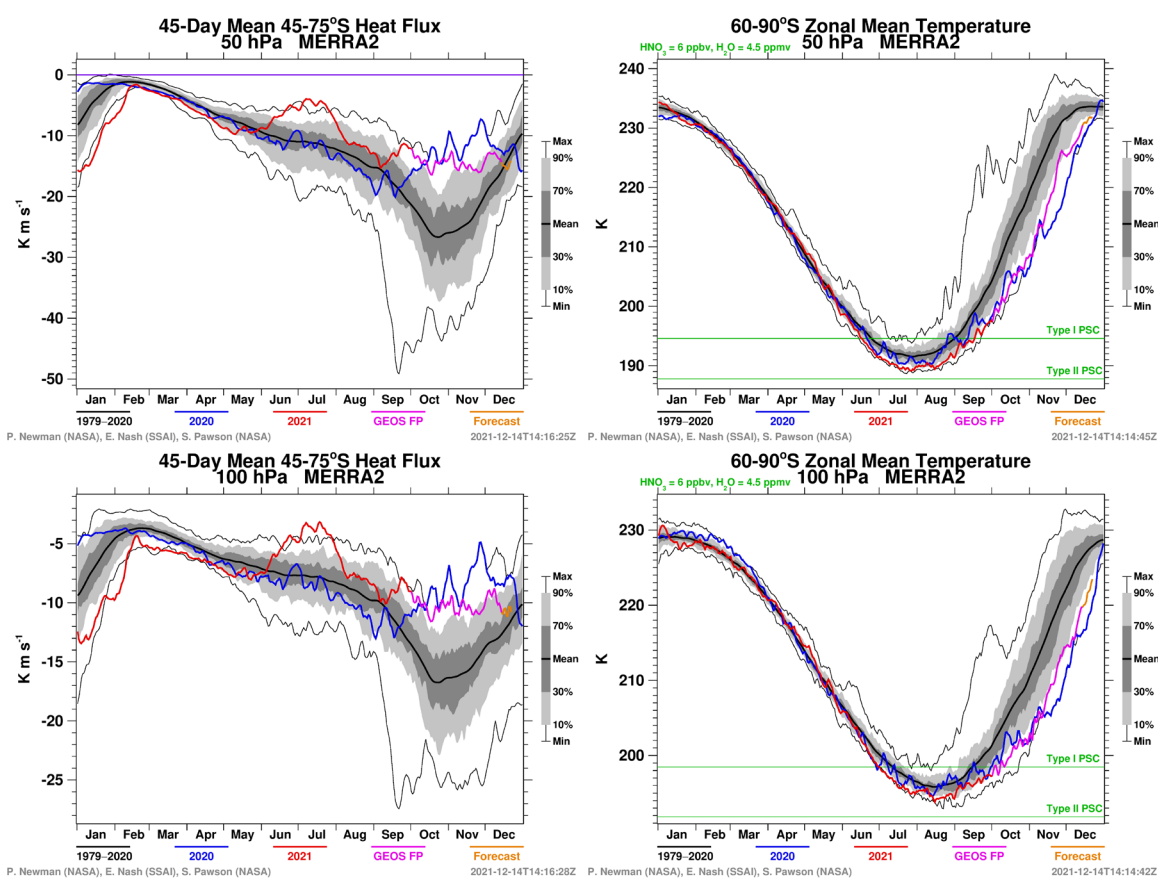
Figure 6 MERRA2 45-day mean 45°S-75°S eddy heat flux and 60°S-90°S zonal mean temperature at 50 & 100 hPa. Images courtesy of NASA GSFC, downloaded 15 December 2021, data through to 22 December 2021 (data starting 2021-10-01 are from GEOS FP; 2021-12-14 onwards are forecasts): http://ozonewatch.gsfc.nasa.gov/meteorology/SH.html
