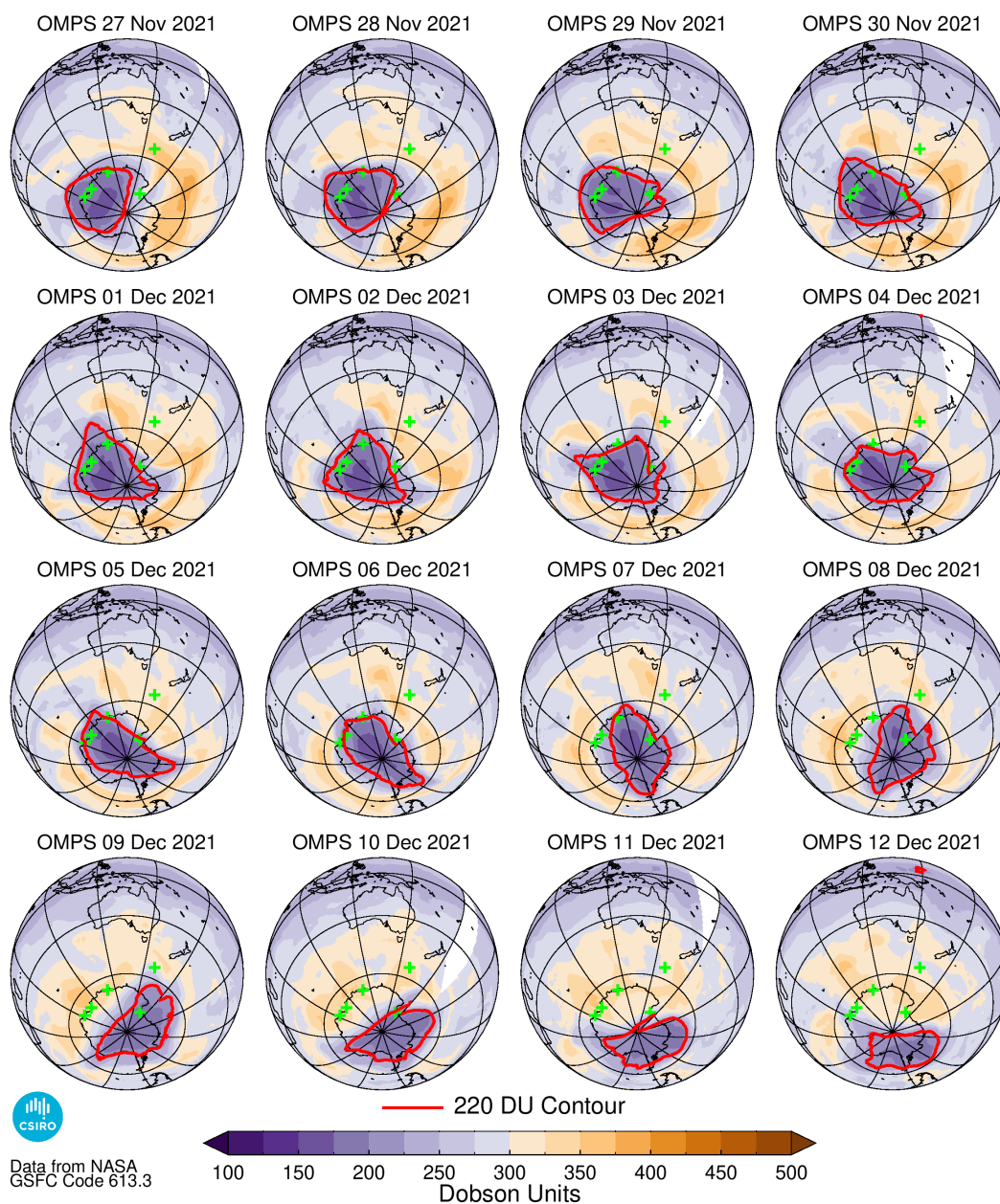
Figure 5 OMPS ozone hole images for 27 November – 12 December; the ozone hole boundary is indicated by the red 220 DU contour line. Green plus symbols indicate the location of the Australian Antarctic stations of Mawson (62.9°E, 67.6°S), Davis (78.0°E, 68.6°S) and Casey (110.5°E, 66.3°S), the New Zealand Antarctic station of Arrival Heights (166.7°E, 77.8°S) and Macquarie Island station (158.9°E, 54.5°S).
