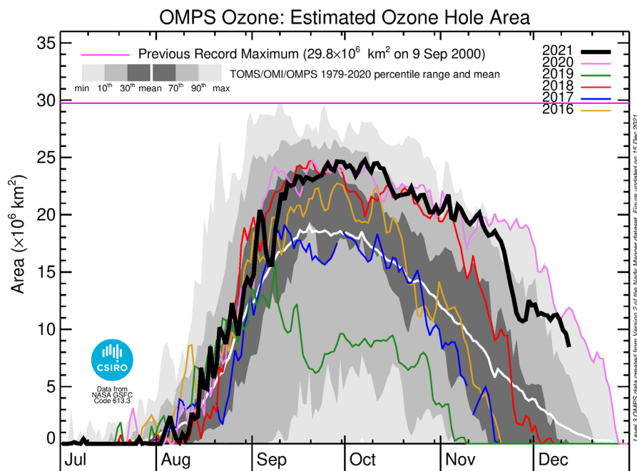
Figure 1 Ozone hole area based on OMPS satellite data (data up to 12 December 2021).
