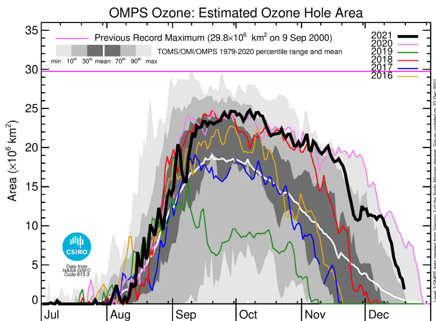
Figure 1 Ozone hole area based on OMPS satellite data (data up to 19 December 2021).
