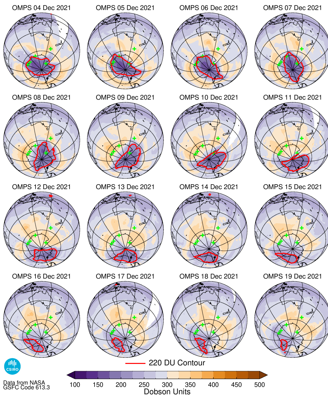
Figure 5 OMPS ozone hole images for 4 – 19 December; the ozone hole boundary is indicated by the red 220 DU contour line. Green plus symbols indicate the location of the Australian Antarctic stations of Mawson (62.9°E, 67.6°S), Davis (78.0°E, 68.6°S) and Casey (110.5°E, 66.3°S), the New Zealand Antarctic station of Arrival Heights (166.7°E, 77.8°S) and Macquarie Island station (158.9°E, 54.5°S).
