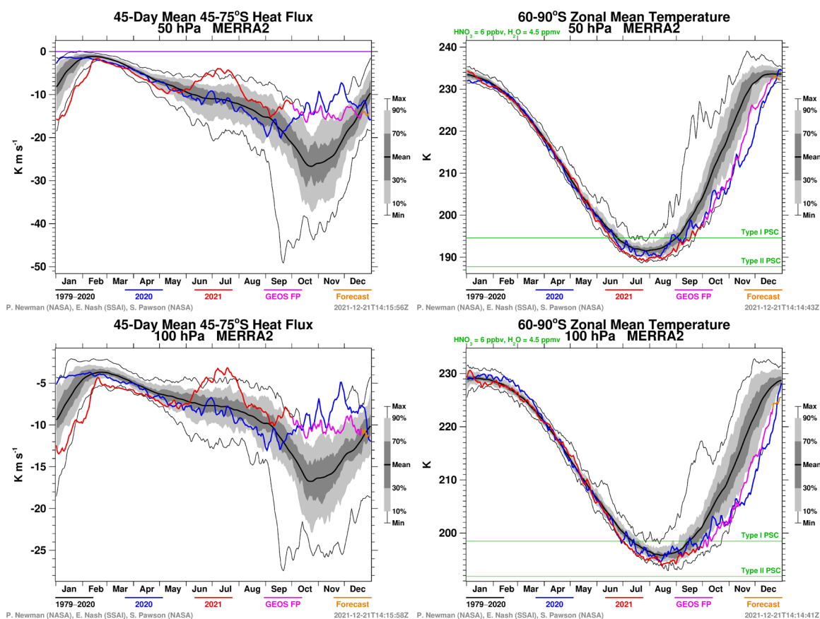
Figure 6 MERRA2 45-day mean 45°S-75°S eddy heat flux and 60°S-90°S zonal mean temperature at 50 & 100 hPa. Images courtesy of NASA GSFC, downloaded 22 December 2021, data through to 29 December 2021 (data starting 2021-10-01 are from GEOS FP; 2021-12-21 onwards are forecasts): http://ozonewatch.gsfc.nasa.gov/meteorology/SH.html
