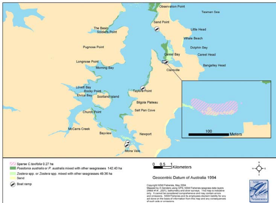
Distribution of Caulerpa taxifolia Careel Bay, Pittwater, August 2003
