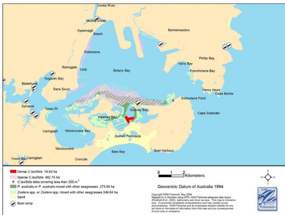
Distribution of Caulerpa taxifolia Botany Bay, March 2004
