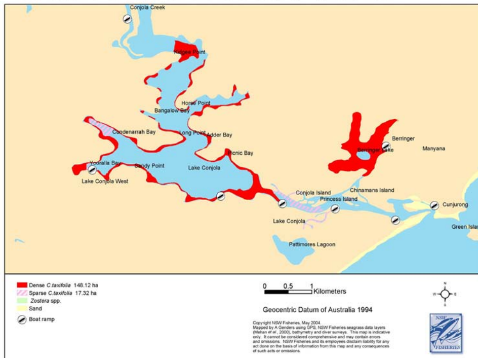
Distribution of Caulerpa taxifolia Lake Conjola, February 2004
