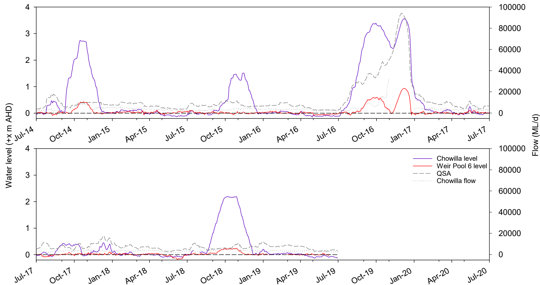
Figure B3. Water levels in Chowilla Creek, downstream of Monomom Creek (+16.4 m AHD), and upstream of Lock 6 (+19.25 m AHD) from 2014–2019, showing Chowilla regulator operations (DEW). Flow to South Australia (QSA) and within Chowilla Creek (calculated as QSA minus flow downstream of Lock 6) are presented.
