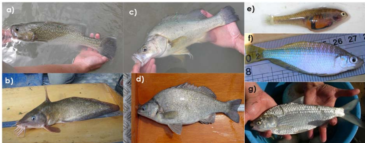
Figure 38. Target species for the LMR: (a) Murray cod and (b) freshwater catfish (equilibrium life history); (c) golden perch and (d) silver perch (periodic life history); and (e) carp gudgeon, (f) Murray rainbowfish and (g) bony herring (opportunistic life history).
