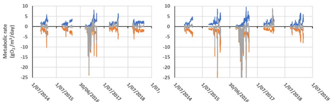
Figure 13. Rates of GPP (●), ER (●) and NEP (●) at (left) Lock 6 and (right) Lock 1 over the five monitoring periods from 2014–2019.
