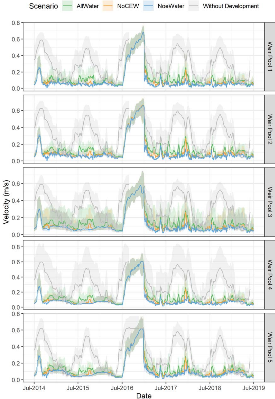
Figure 8. Median modelled velocity in each weir pool (line), with the range in velocities within the weir pool (the shaded area), defined by the 10 th and 90 th percentiles, in the LMR.
