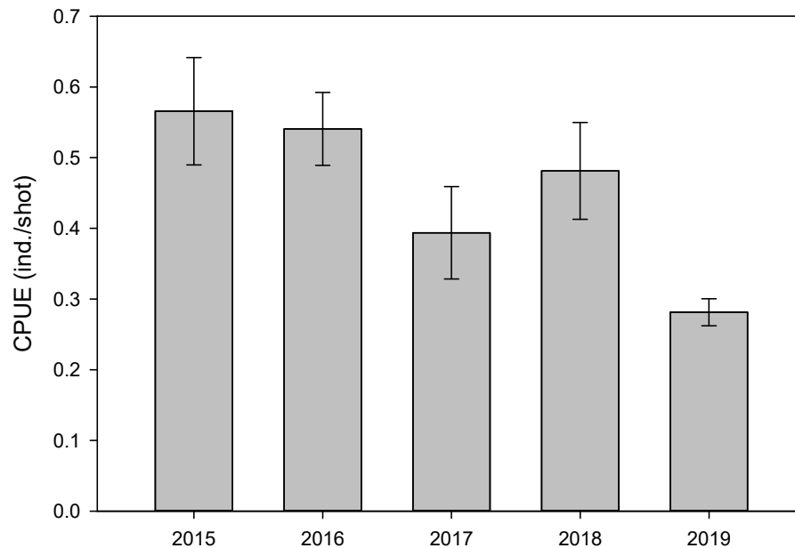
Figure 35. Mean catch-per-unit-effort (CPUE) \pm standard error of golden perch captured during Category 1 Fish Assemblage electrofishing (individuals per 90 second shot) in the gorge geomorphic zone (10 sites) of the LMR in autumn from 2015–2019. CPUE data from five sites are presented for 2017 as other sites were sampled during winter 2017.
