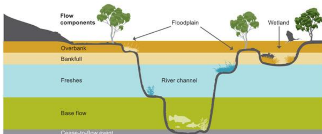
Figure 3.1. The various flow types as described by the Murray–Darling Basin Plan and Gawne et al. (2013a).
