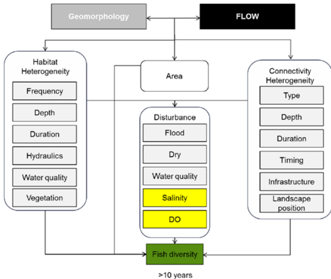
Figure 4.3. Fish (Channel) cause and effect diagram (MDFRC 2013). Magnitude, timing and duration are factors of flow (in black).
