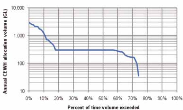
Figure 10-5: Distribution of annual Commonwealth allocation required to achieve all ecological targets, with allocation of 300 GL/year with no carryover.
