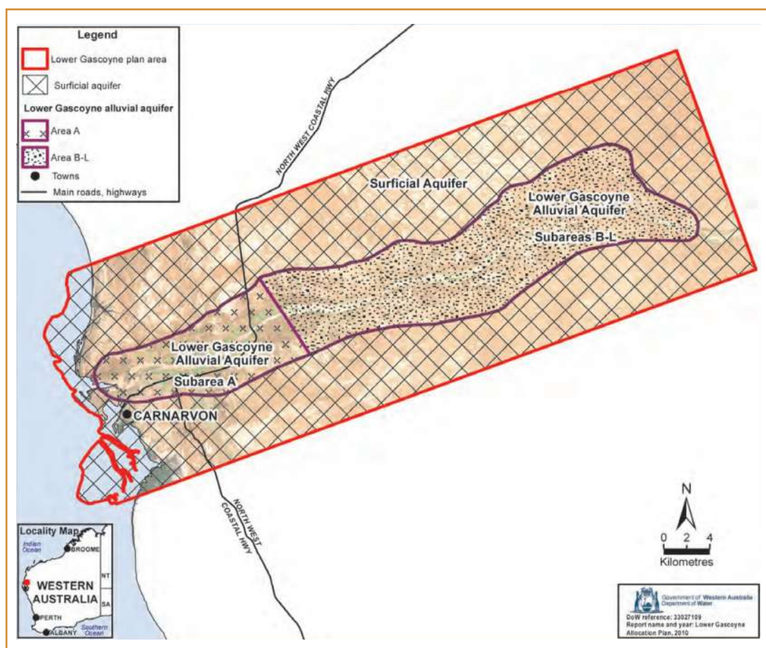
Figure 10: Resource boundaries used in the Lower Gascoyne water allocation plan.
