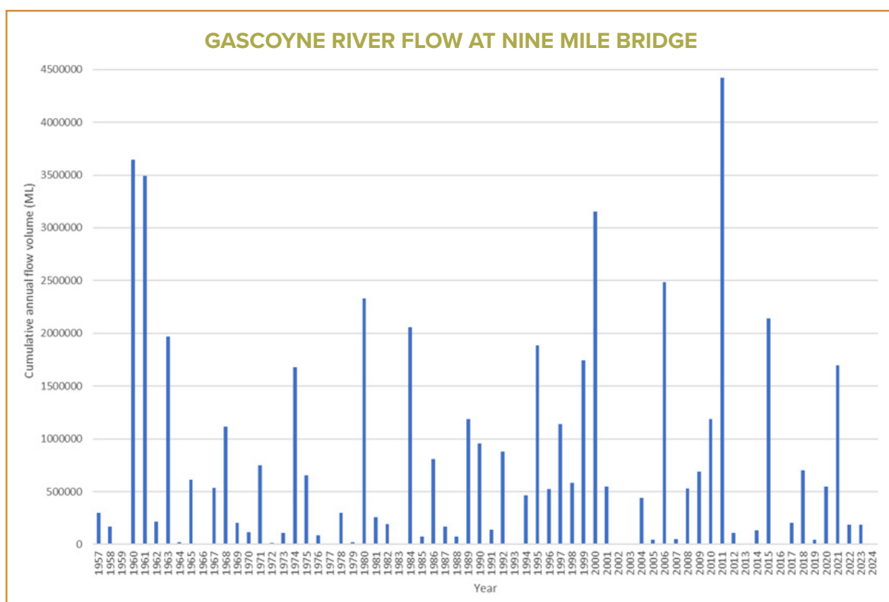
Figure 7: Gascoyne River total annual discharge at Nine Mile Bridge
