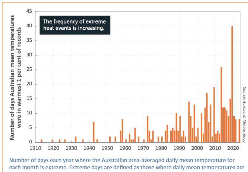
Figure 16: Increase of extreme temperature days in Australia (CSIRO and Australian Government Bureau of Meteorology, 2024).
