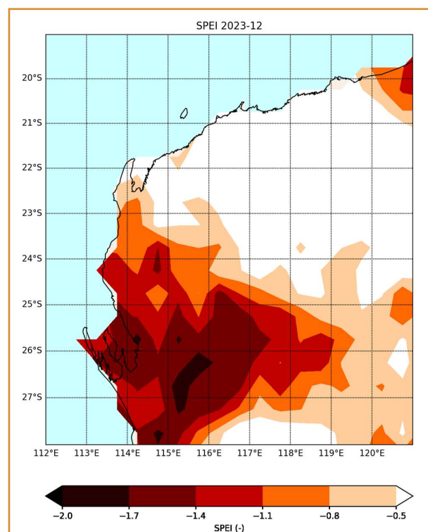
Figure 11: Standardised Precipitation Evaporation Index (SPEI) for Gascoyne region in December 2023.
