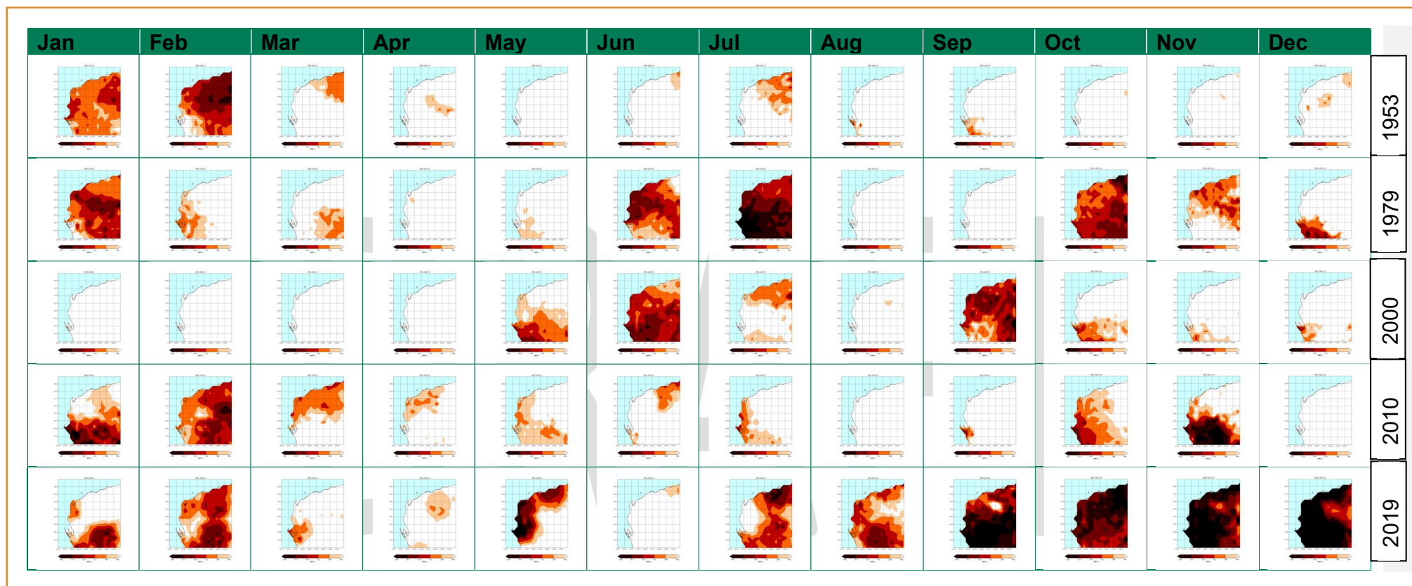
Figure 14: Monthly SPEI for 1953, 1979, 2000, 2010 and 2019 for the Gascoyne region.
