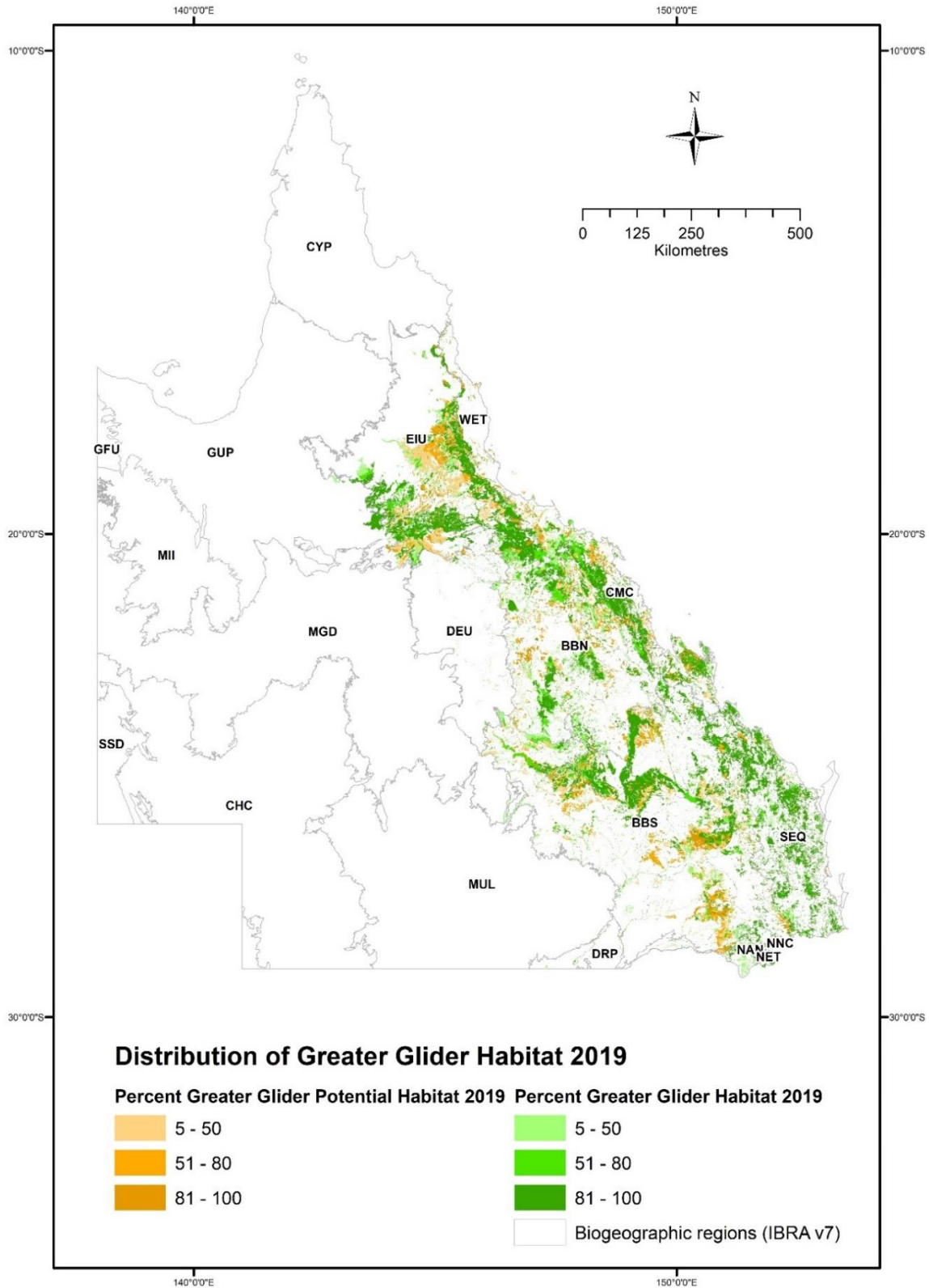
Map 3 Distribution of greater glider potential habitat and habitat throughout Queensland, using remnant (at 2019) regional ecosystems
