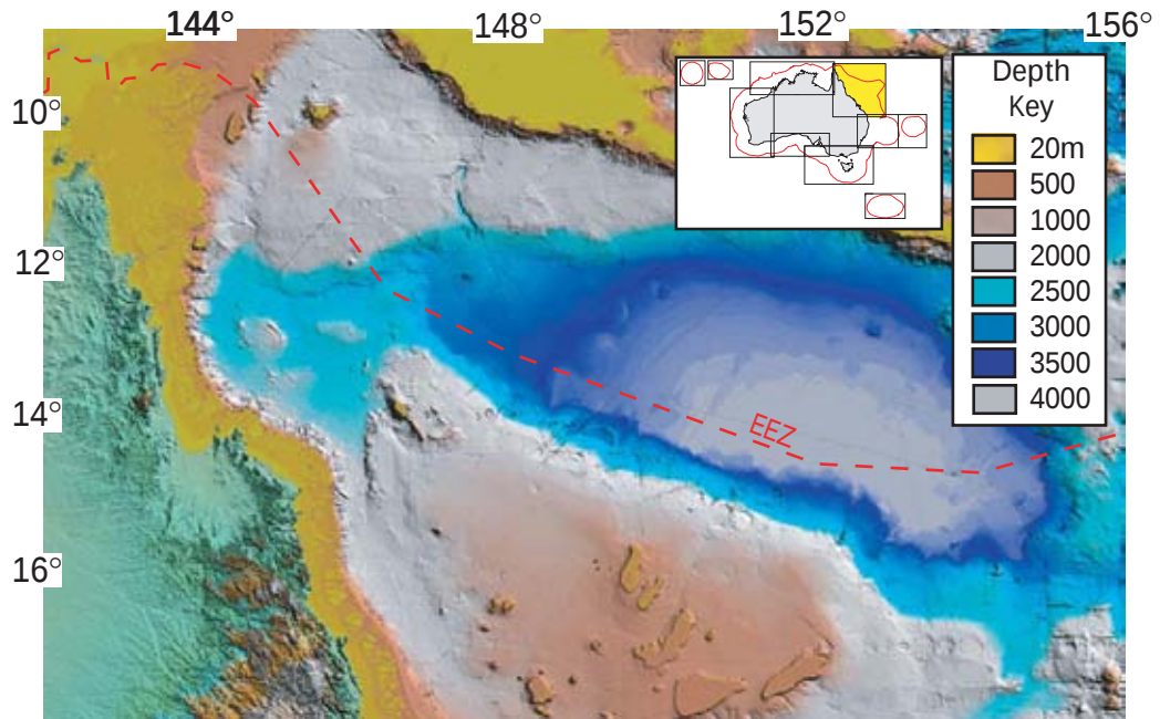
Figure 3.20. False-colour bathymetric image illuminated from the north showing the northeast margin with the Coral Sea basin and marginal plateaus.
