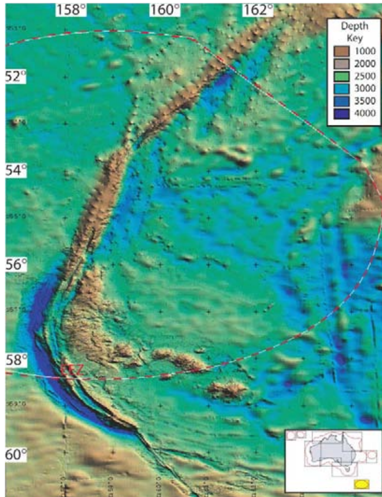
Figure 3.33. False-colour bathymetric image illuminated from the north of the Macquarie Island margin. The Hjord Trench, up to 6,000 m deep, extends across the southwestern part of the image.
