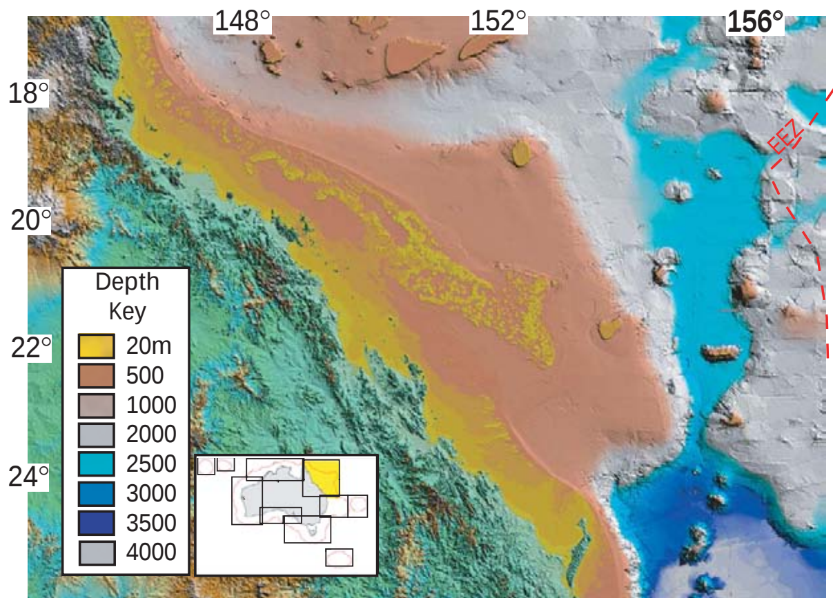
Figure 3.21. False-colour bathymetric image illuminated from the north showing the northeast margin with the northern Tasman Sea basin and marginal plateaus.
