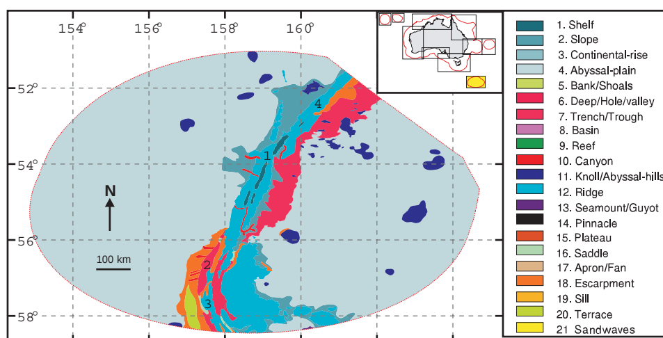
Figure 3.32. Geomorphic features of the Macquarie Island margin. See Table 3.17 for key to place names and Table 3.18 for surface areas of features.
