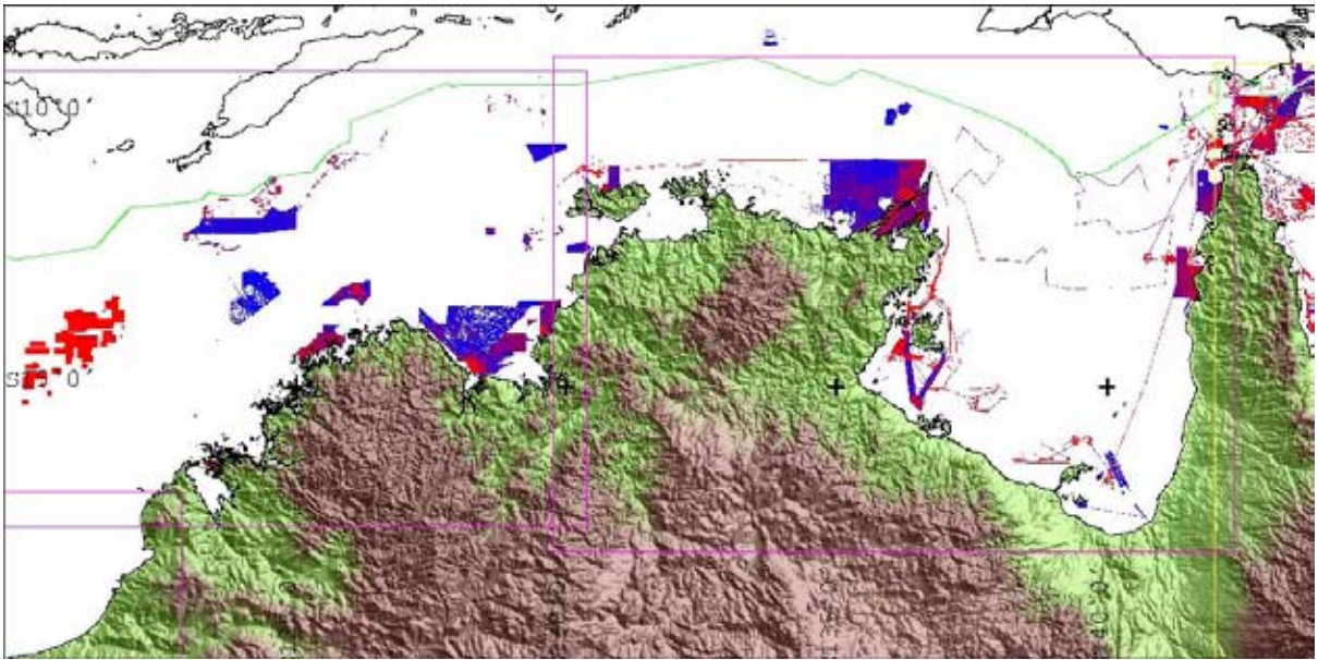
Figure 2.2. Bathymetric data added to the Geoscience Australia database. (A) Northern margin. Red >200 data points \text{km}^{-2} (LADS, Multibeam sonar datasets and high density vertical soundings); Purple 20-200 data points \text{km}^{-2} ; Blue <20 data points \text{km}^{-2} (Vertical soundings and digitised fair sheets).
