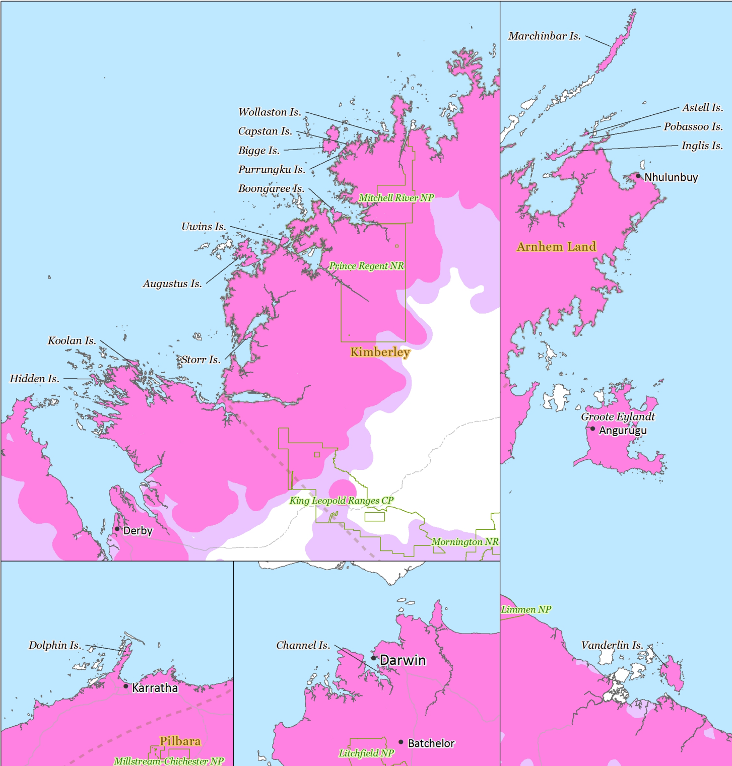
Map 5: The modelled distribution of northern quoll ( Dasyurus hallucatus ) on islands in Western Australia and the Northern Territory (as at February 2011)
