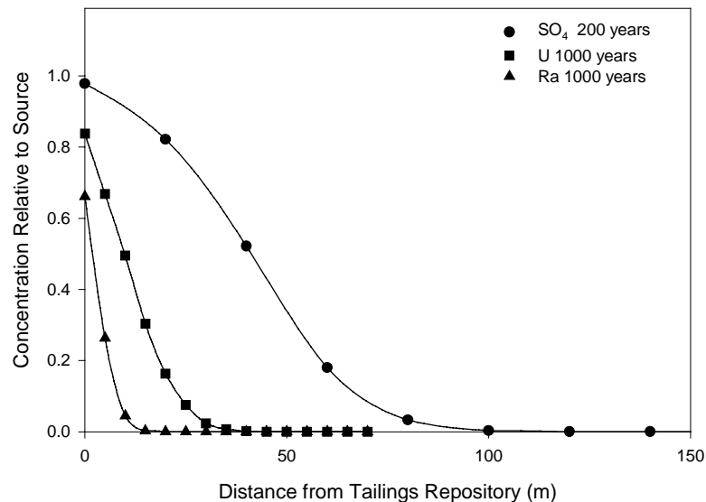
Figure 5.3.5 Variation of the median concentrations of SO 4 , U and Ra with distance east of the tailings silos at Jabiluka. Concentrations are expressed as ratios to the 'source' concentration immediately downstream of the silos. The SO 4 concentrations were calculated 200 years after placement. The U and Ra concentrations were calculated 1000 years after placement.
