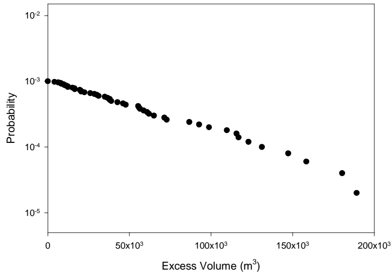
Figure 4.3.1 Probability of occurrence of excess water volumes in the Jabiluka Total Containment Zone over the life of the mine for the storage capacity specified by ERA
