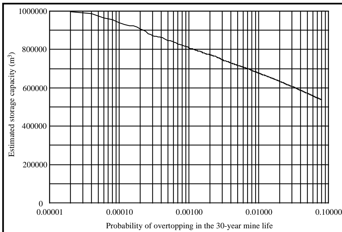
Figure 4.2.1 Estimates of storage capacity required as a function of exceedence probability over the 30-year mine life under current climatic conditions
