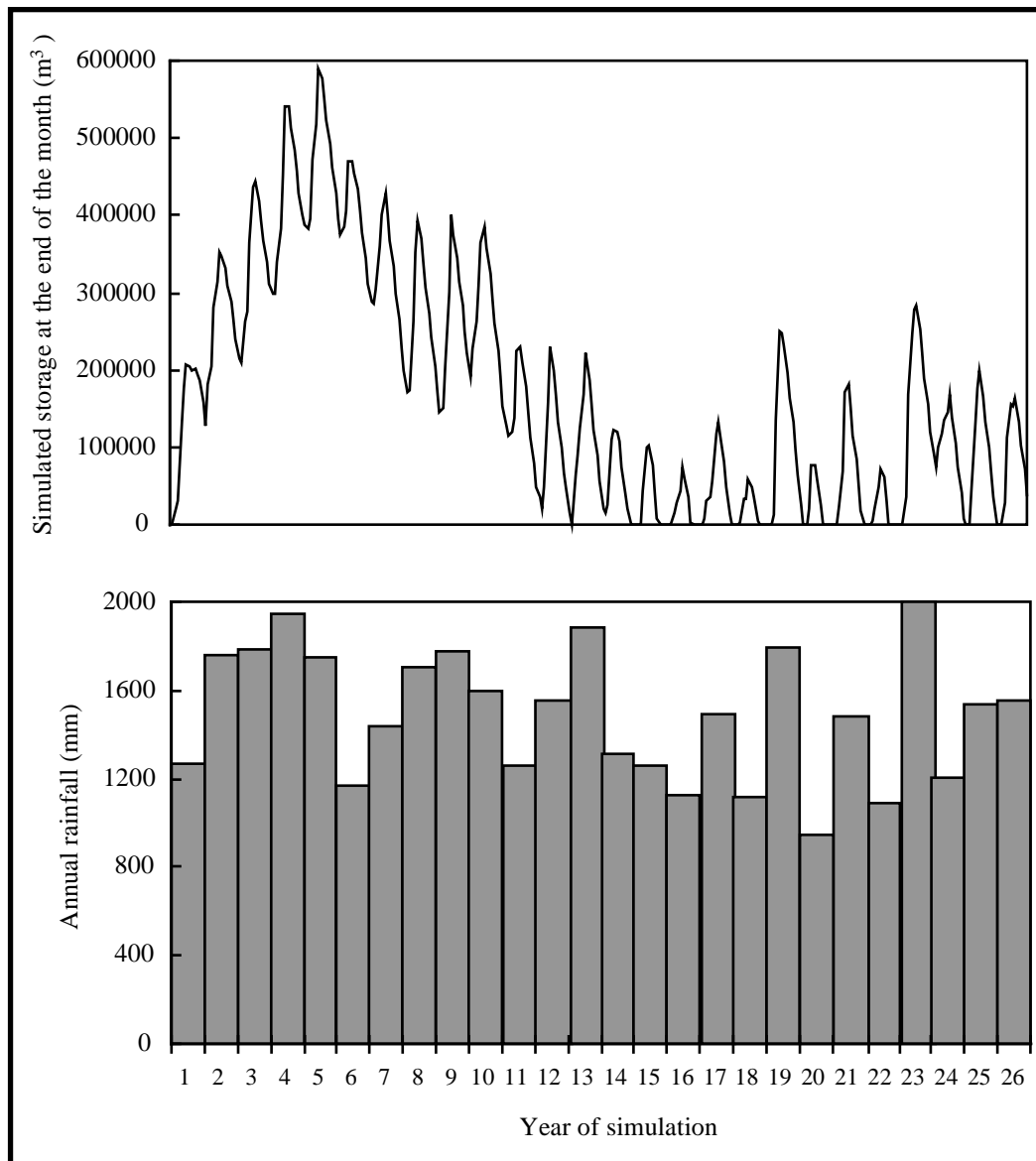
Figure 4.2.2 Annual rainfall (September–August) and accumulated water volumes for a model simulation using actual rainfall and evaporation from September 1972 to August 1998
