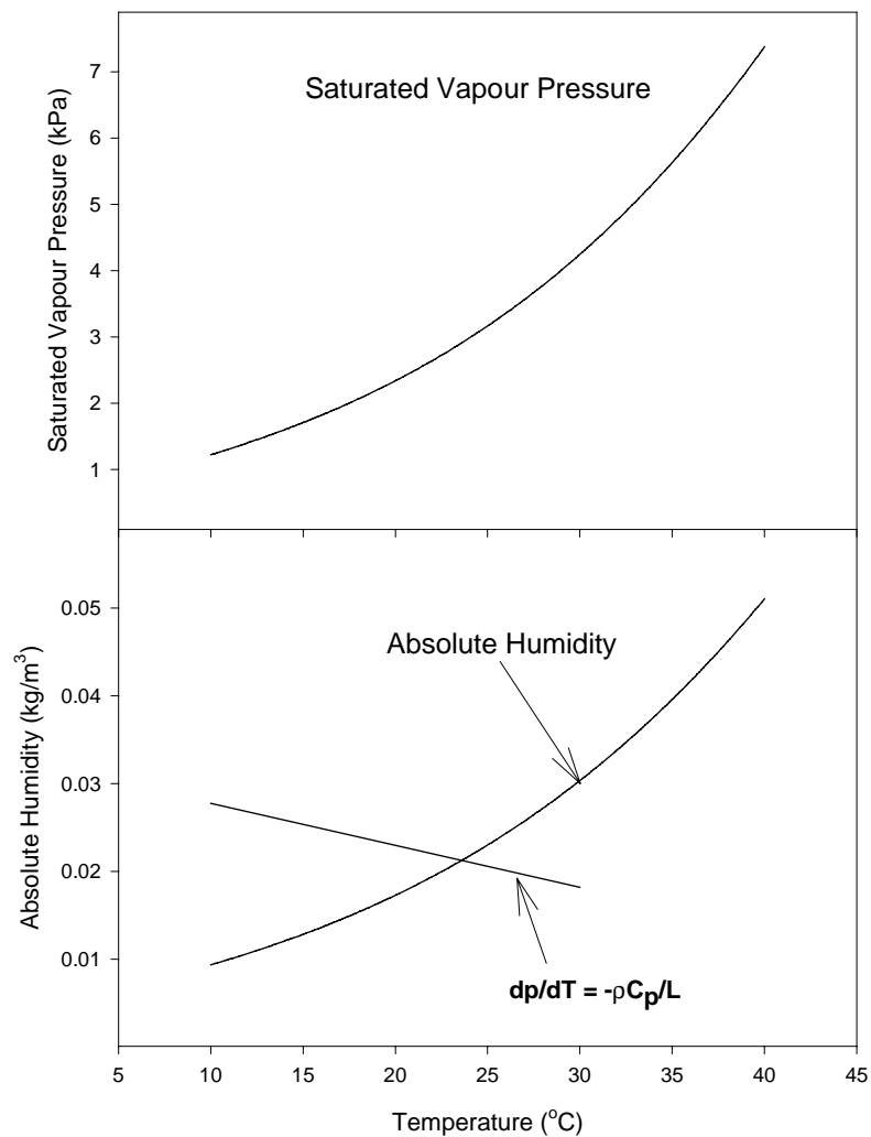
Figure 2.4.1 Variation of saturated vapour pressure (upper graph) and absolute humidity (lower graph) with temperature at atmospheric pressure P=100 kPa
