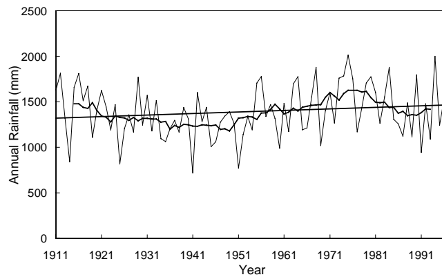
Figure 3.4.2 Average annual rainfall from Oenpelli 1911–1997, showing a 10-year moving average and linear trend of 1.7 mm pa
