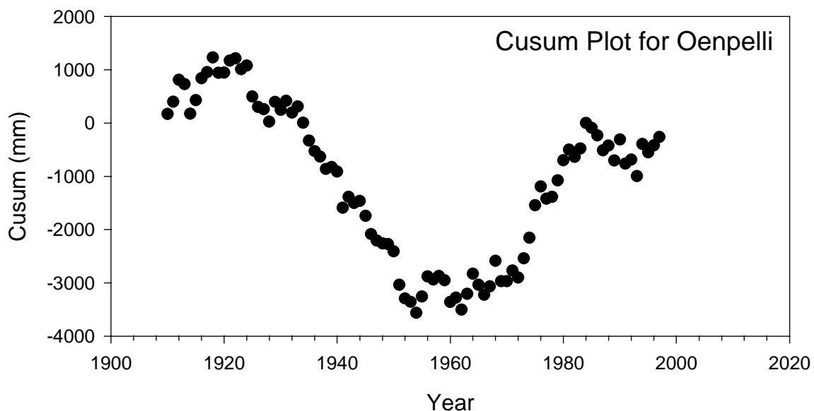
Figure 3.4.1 Cusum plot for the annual rainfall records at Oenpelli showing low average rainfall from 1932–1952 and high average rainfall from 1970–1984
