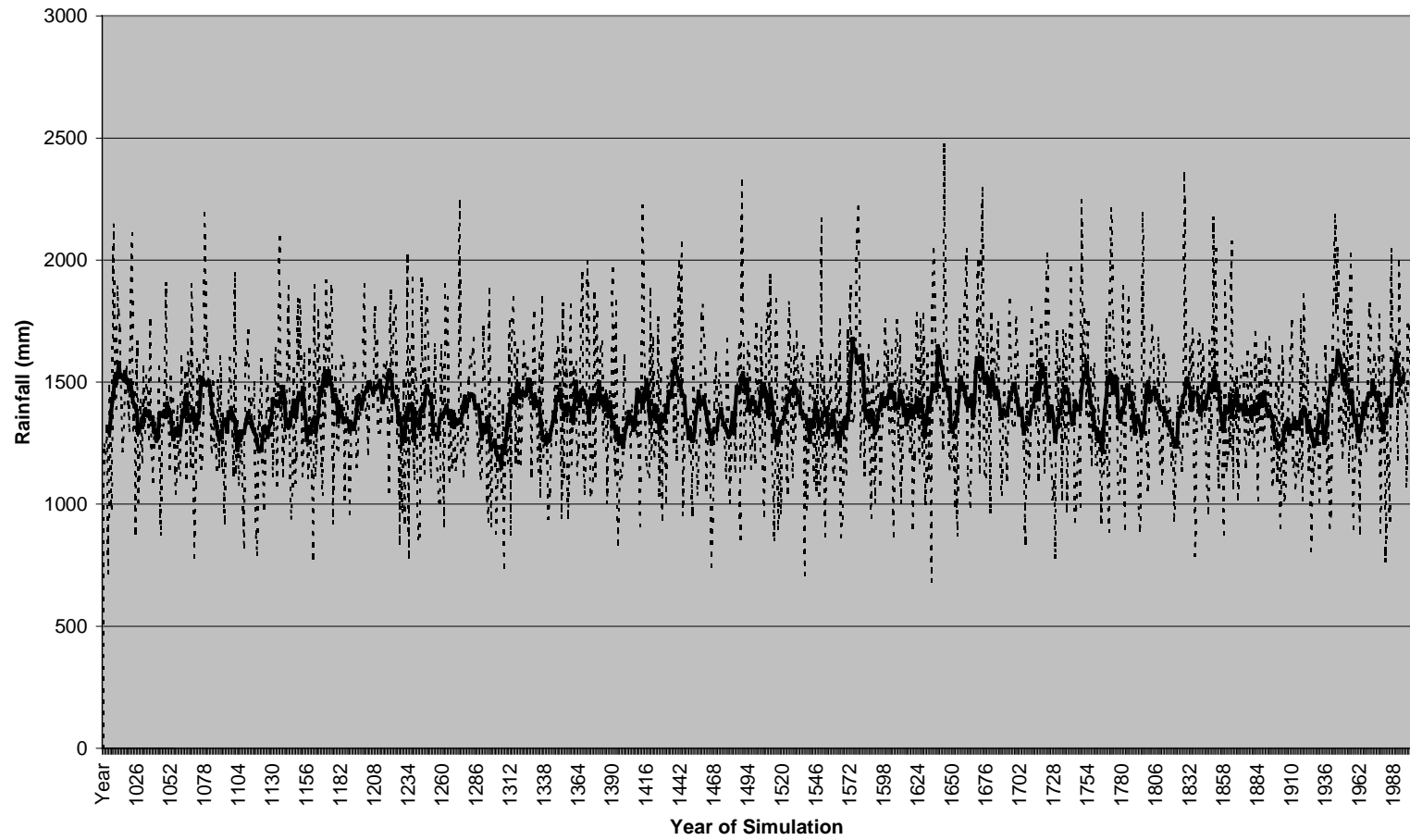
Figure 3.4.3 Examination of 1000 years of simulated rainfall data to determine the extent to which decadal scale variation is present
