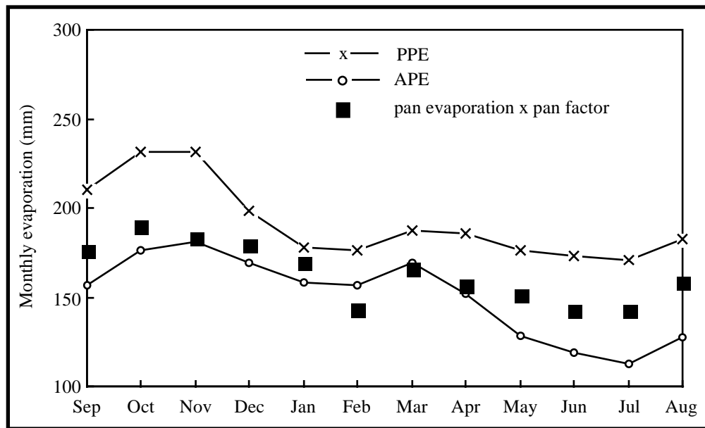
Figure 2.3.1 Comparison of average monthly storage evaporation estimates and point potential and areal potential evapotranspiration rates
