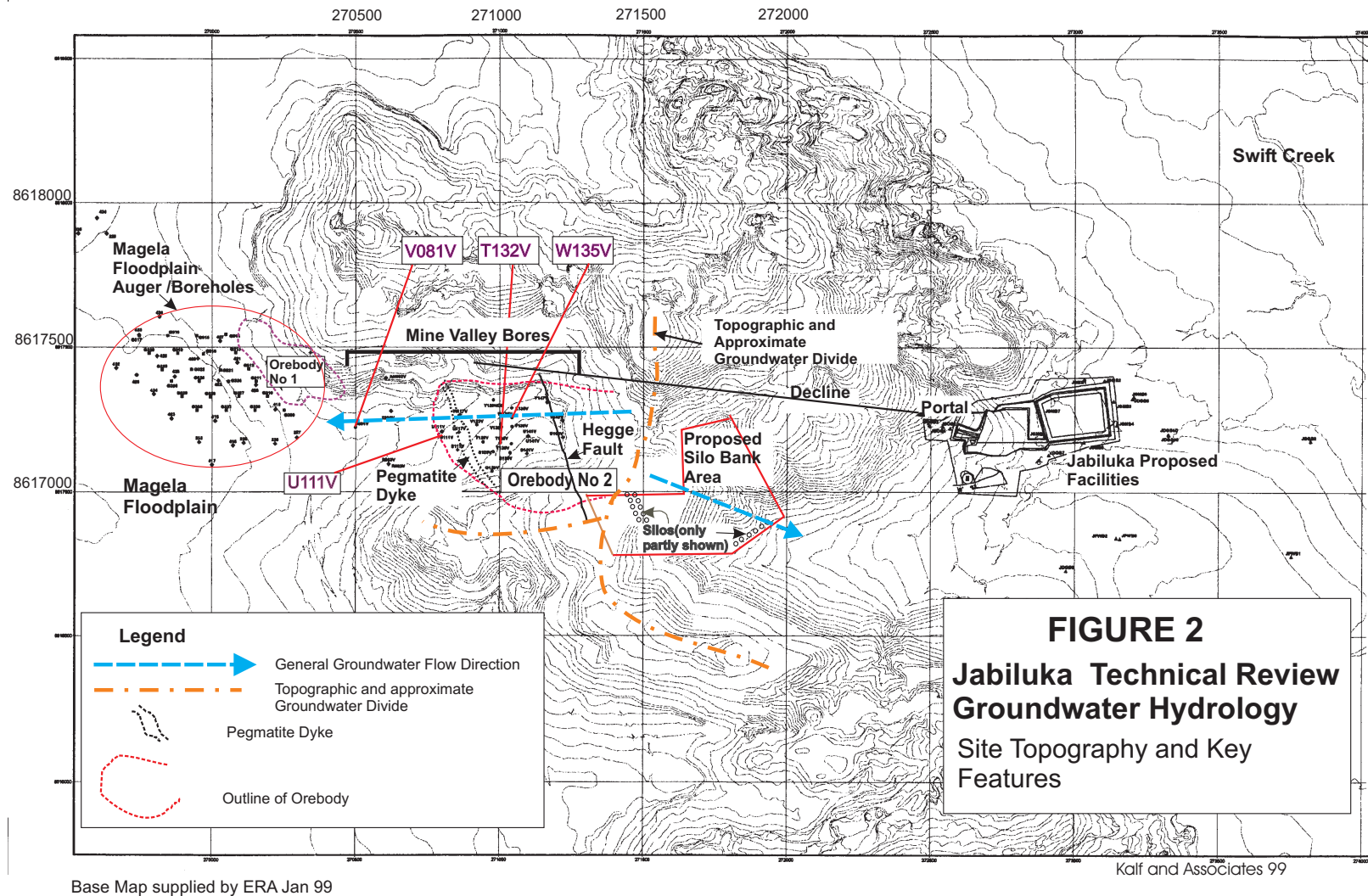
Figure 5.3.2 Topography and key hydrogeological features of the Jabiluka area
