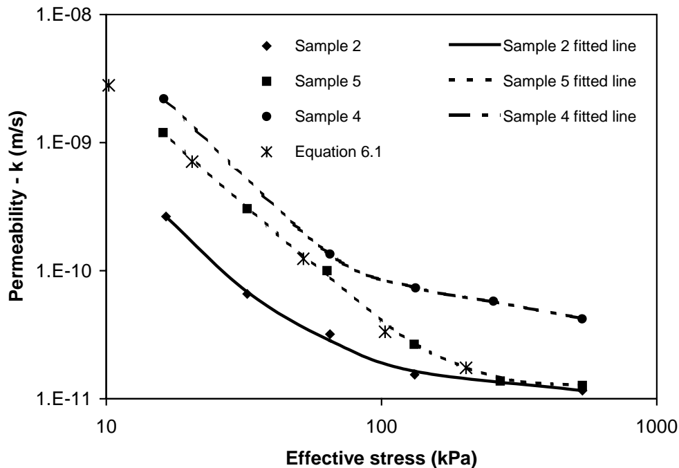
Figure 5.3.4 Permeability (m/s) as a function of effective stress (kPa) for tailings from the Ranger mine located 22 km from Jabiluka
