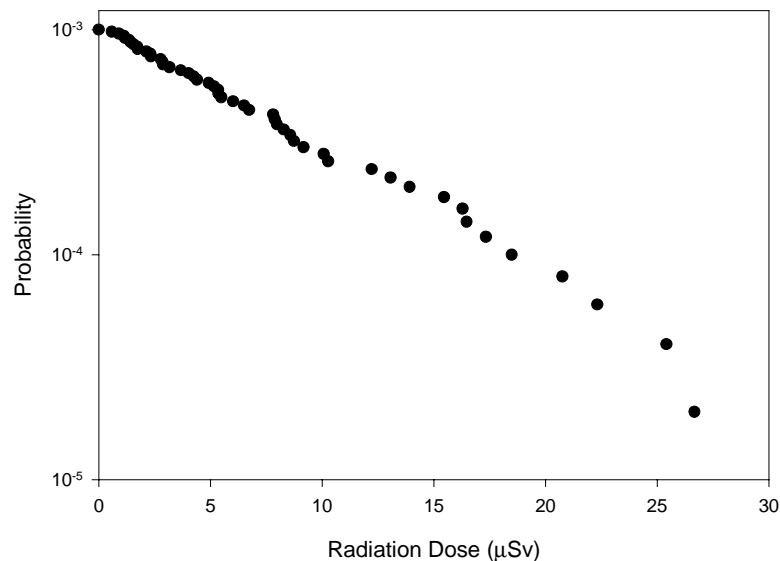
Figure 4.3.2 Probability versus radiation exposure of members of the public resulting from the discharge of excess water from the Jabiluka mine site for the water management system proposed by ERA
