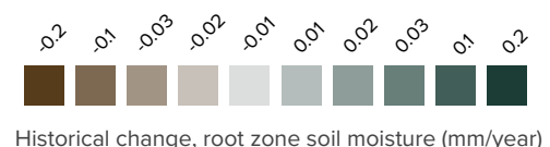
Figure 26: Changes in conditions during drought against a present-day baseline of 2002 to 2022
