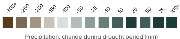
Figure 26: Changes in conditions during drought against a present-day baseline of 2002 to 2022
