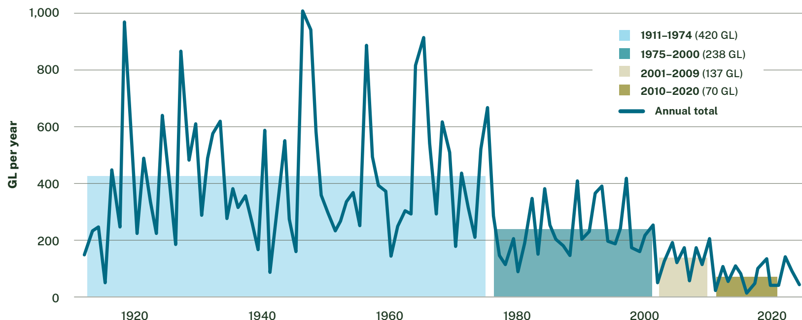
FIGURE 3 Reduction in streamflow into water reservoirs supplying Perth and South West regions over the past 100 years.
