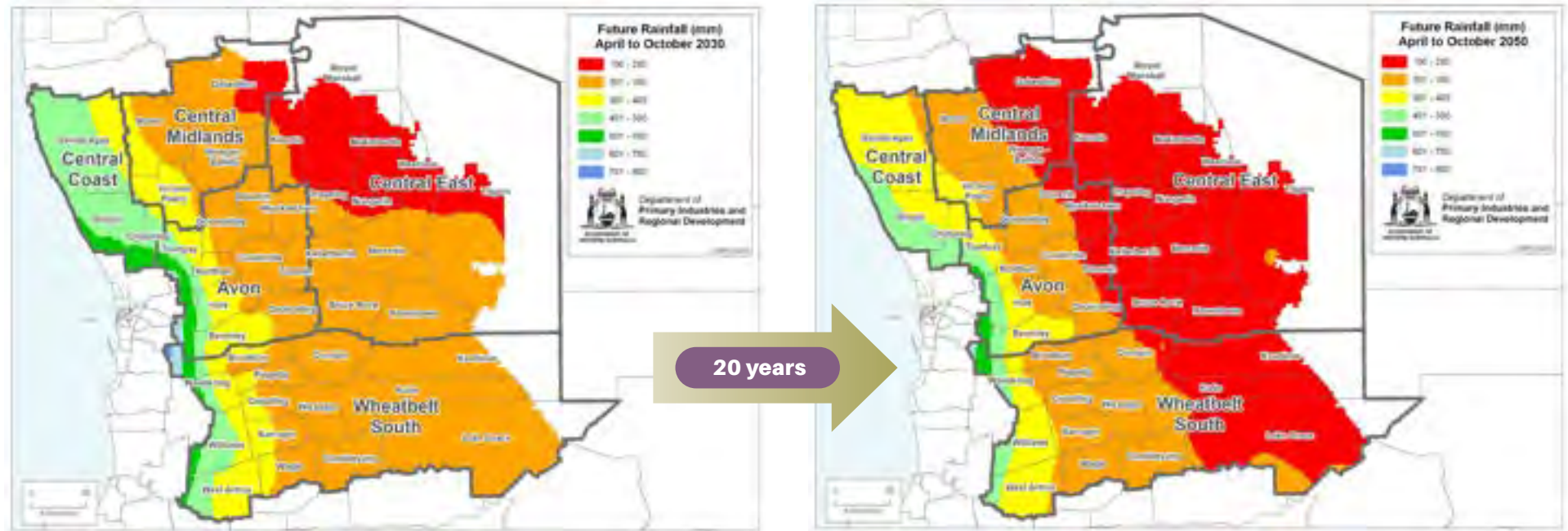
FIGURE 6 Predicted growing season rainfall across the Wheatbelt in 2030 and 2050 compared with recent past. Note: Predictions are based on a medium emissions scenario in which greenhouse gas emissions are reduced substantially by end of the century, but not enough to stop continued warming.
