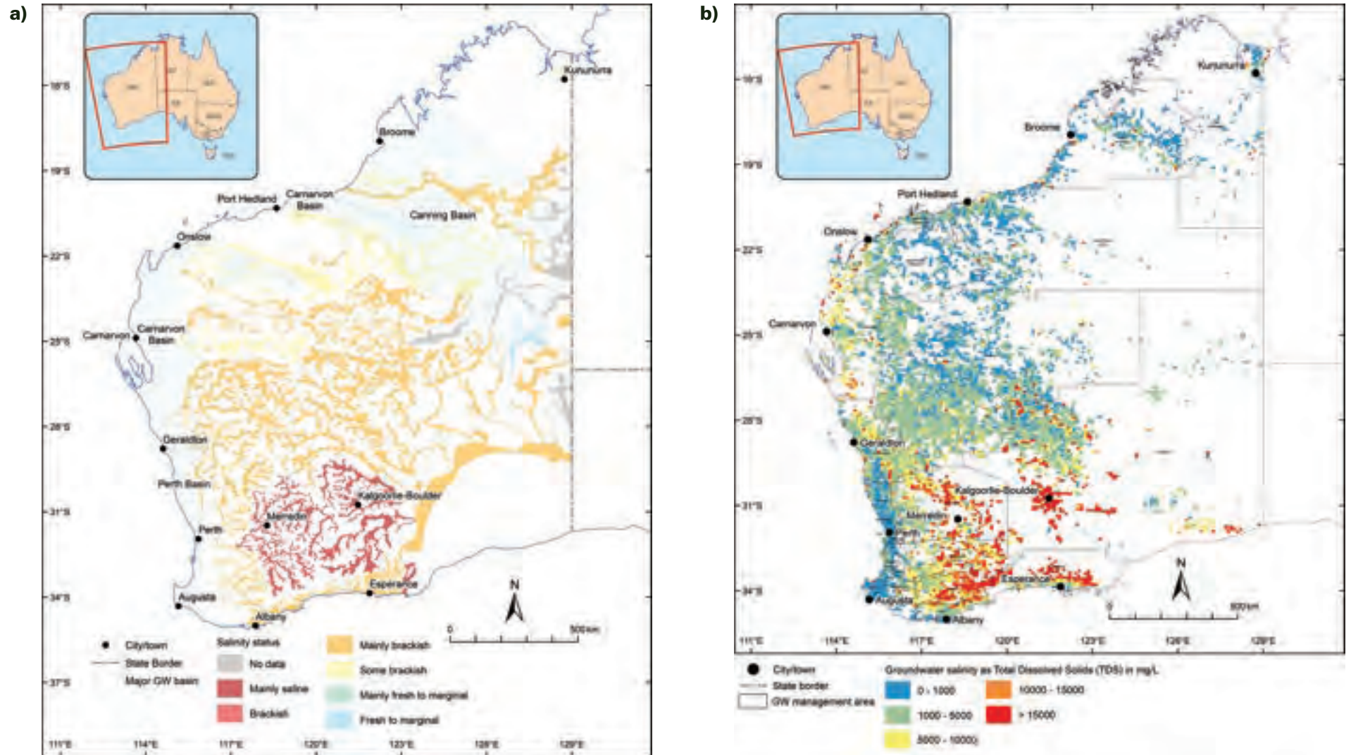
FIGURE 20 Salinity levels of groundwater systems across Western Australia. Note: most of the Wheatbelt has access to some form of brackish to saline groundwater (seawater is 35,000 mg/litre).
