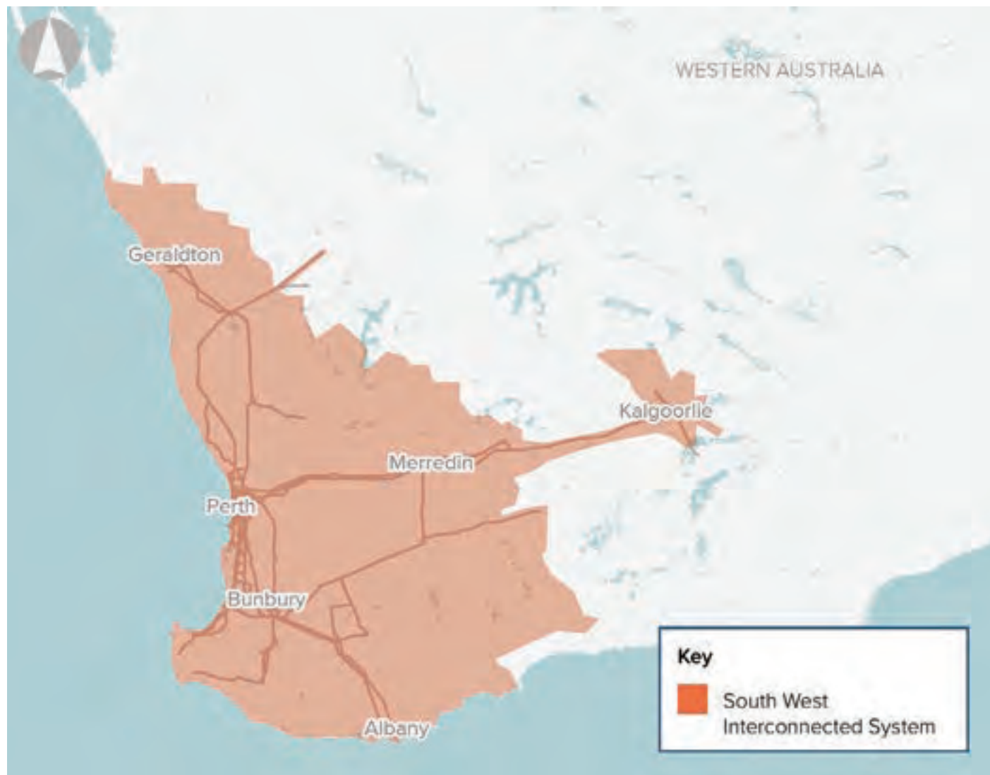
FIGURE 5 Geographic spread of the 7,750 kilometres of transmission lines that make up the South West Interconnected System (SWIS) for electricity production and distribution. A further 90,000+ kilometres of distribution lines (not shown) feed off the transmission line network to deliver electricity into Wheatbelt communities.
