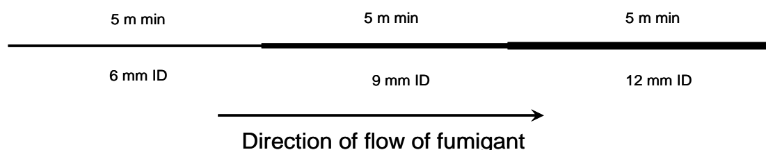
Figure 2 Copper tubing with progressively increasing diameter to avoid back pressure
