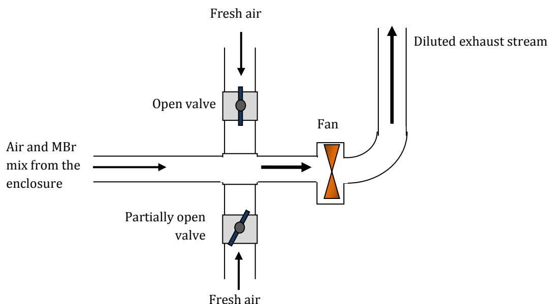
Figure 7 Example of a ventilation/exhaust system for a fumigation chamber
