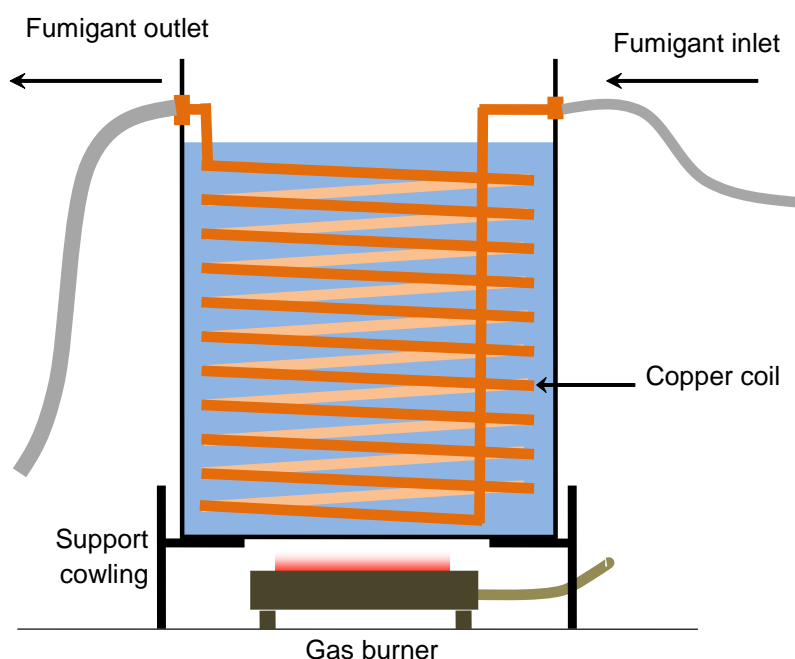
Figure 3 A conventional vaporiser using coiled copper tubing in heated water
