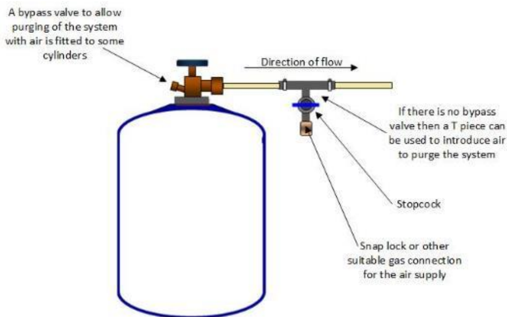
Figure 1 Illustration of a gas cylinder supply system for methyl bromide
