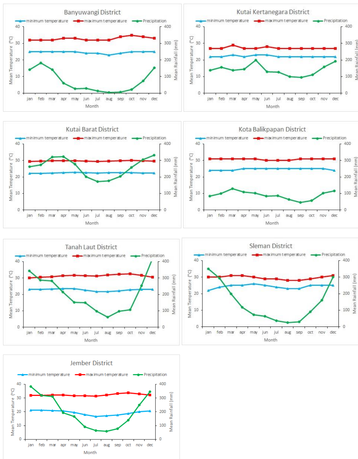
Figure 2 Mean monthly maximum and minimum temperatures and mean monthly rainfall in main dragon fruit production districts
