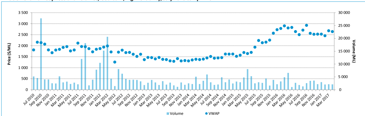
Entitlement market prices and volumes, Goulburn, high reliability, July 2010 to April 2017
