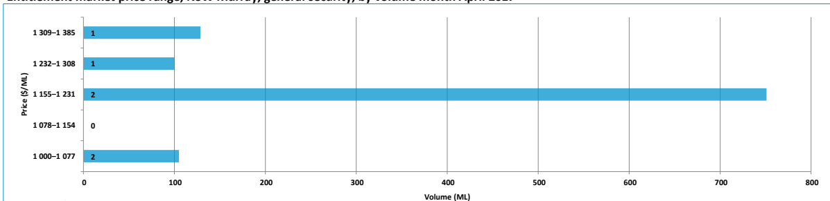
Entitlement market price range, NSW Murray, general security, by volume month April 2017
