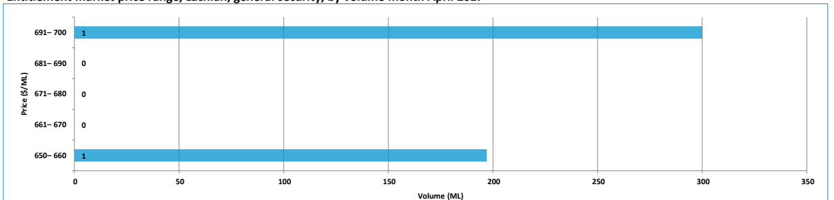
Entitlement market price range, Lachlan, general security, by volume month April 2017
