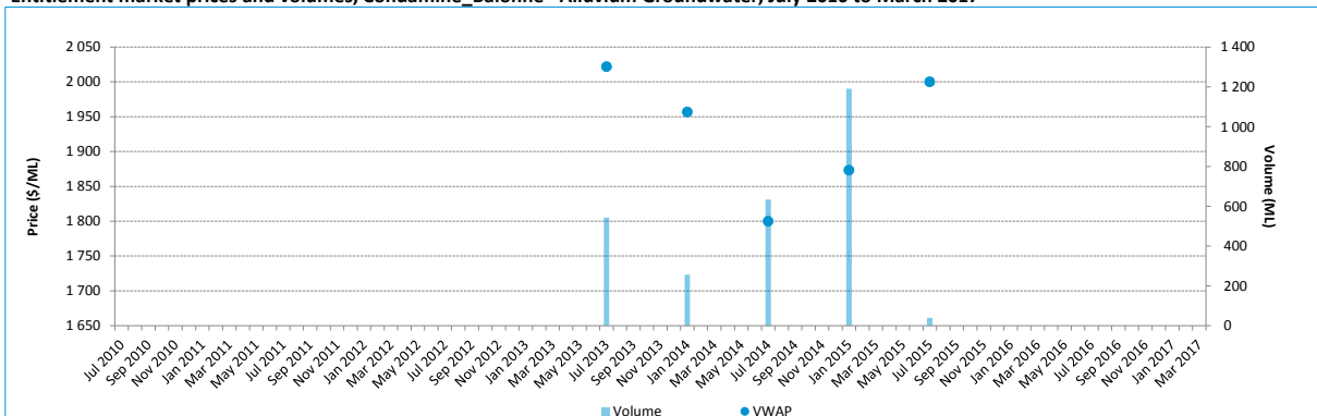
Entitlement market prices and volumes, Condamine_Balonne - Alluvium Groundwater, July 2010 to March 2017
