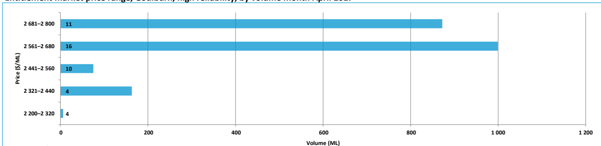
Entitlement market price range, Goulburn, high reliability, by volume month April 2017
