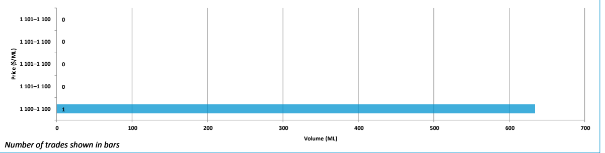
Entitlement market price range, Barwon–Darling, unregulated, by volume month April 2017
