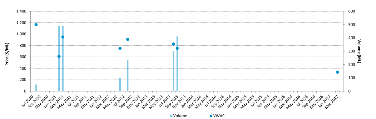
Entitlement market prices and volumes, Lower Darling, general security, July 2010 to April 2017
