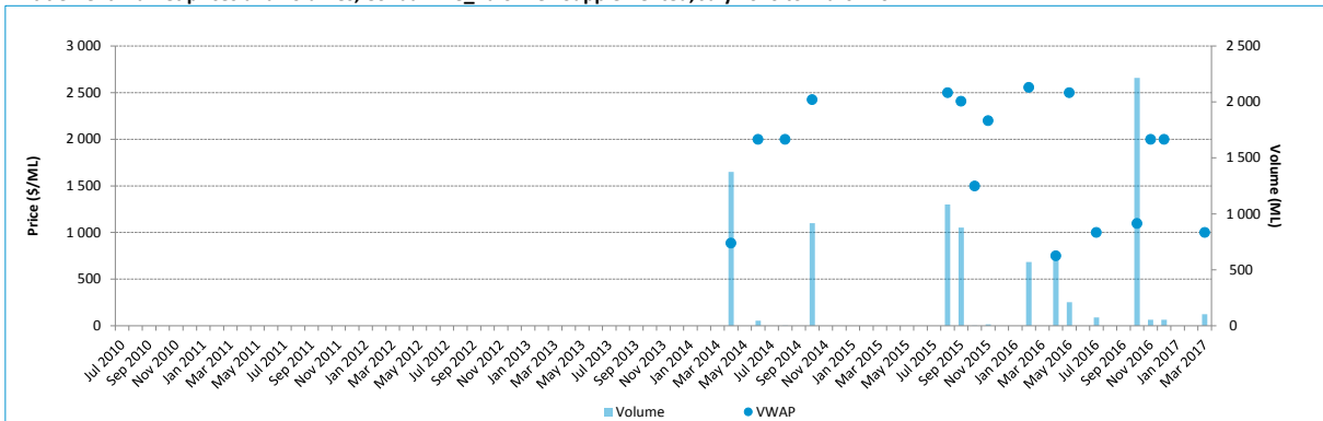
Entitlement market prices and volumes, Condamine_Balonne - Supplemented, July 2010 to March 2017
