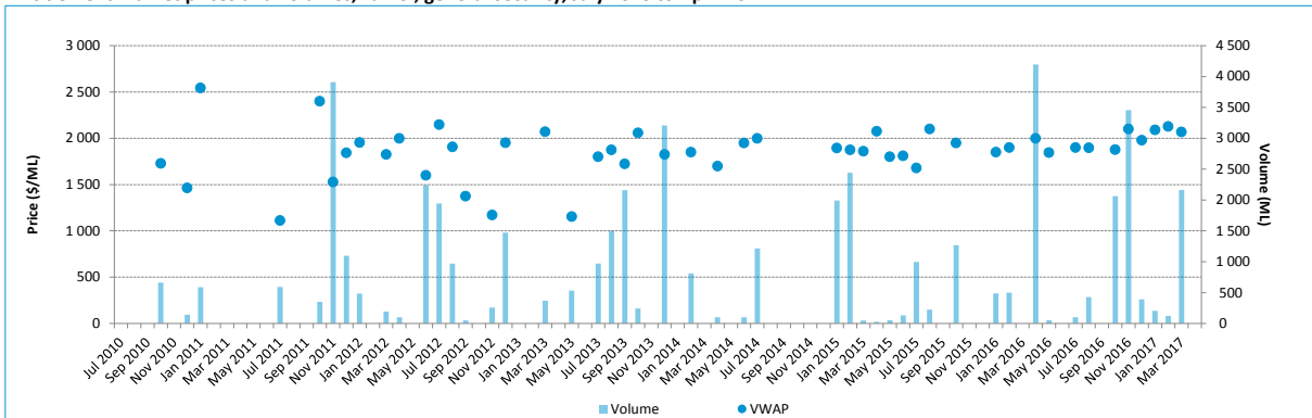
Entitlement market prices and volumes, Namoi, general security, July 2010 to April 2017
