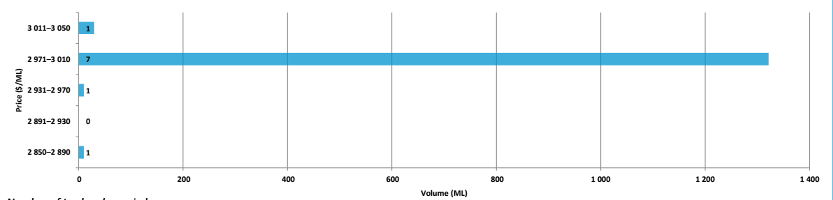
Entitlement market price range, SA Murray, Class 3a, by volume month April 2017
