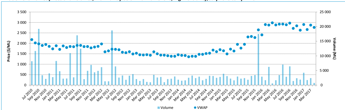
Entitlement market prices and volumes, Vic. Murray below Barmah Choke, high reliability, July 2010 to April 2017
