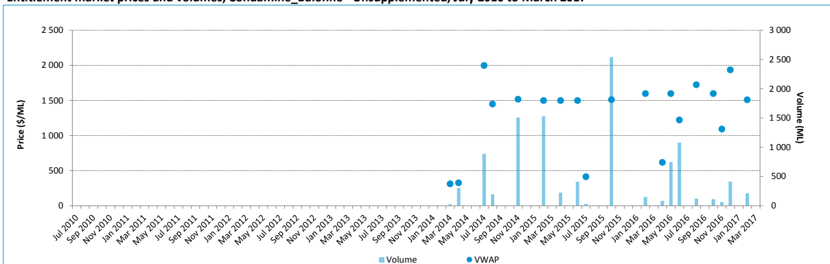
Entitlement market prices and volumes, Condamine_Balonne - Unsupplemented, July 2010 to March 2017
