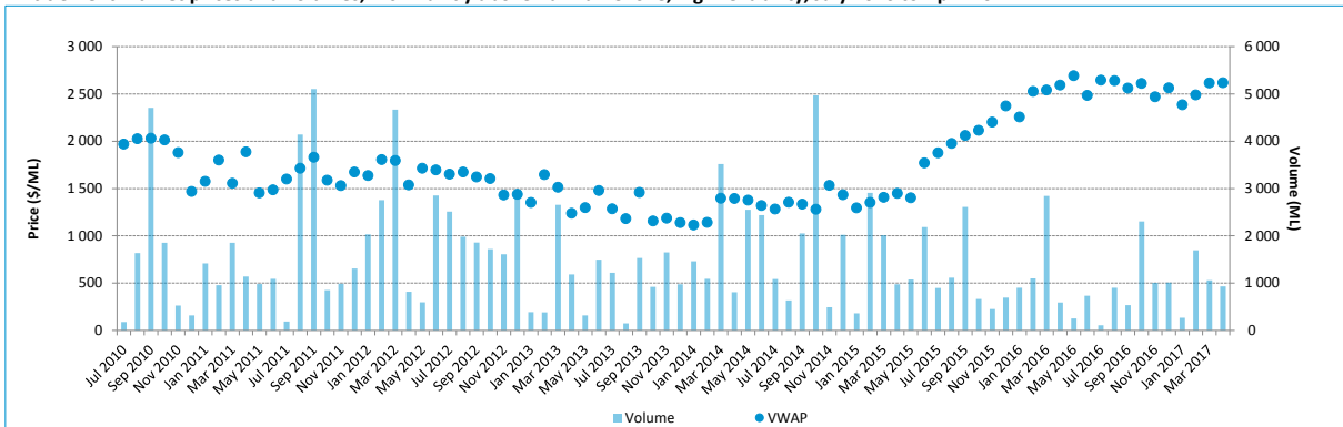
Entitlement market prices and volumes, Vic. Murray above Barmah Choke, high reliability, July 2010 to April 2017
