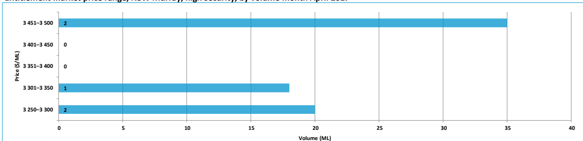
Entitlement market price range, NSW Murray, high security, by volume month April 2017
