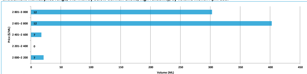
Entitlement market price range, Vic. Murray below Barmah Choke, high reliability, by volume month April 2017
