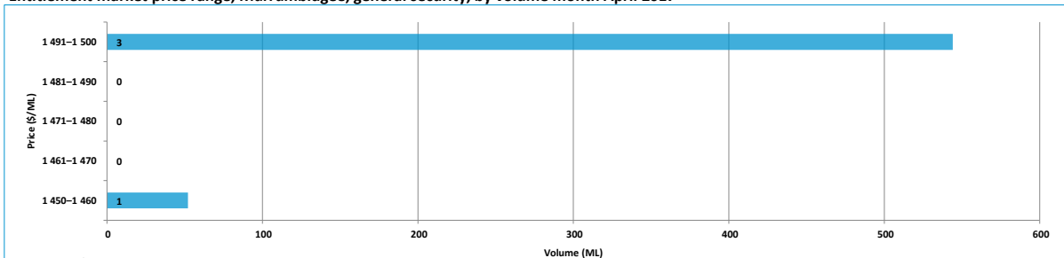
Entitlement market price range, Murrumbidgee, general security, by volume month April 2017
