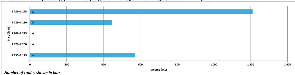
Entitlement market price range, NSW Murray Irrigation Limited, general security, by volume month April 2017
