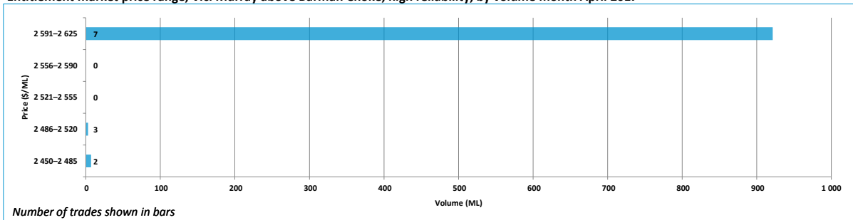
Entitlement market price range, Vic. Murray above Barmah Choke, high reliability, by volume month April 2017
