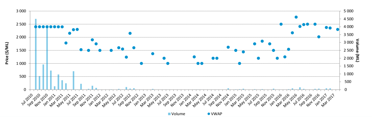
Entitlement market prices and volumes, Campaspe, high reliability, July 2010 to April 2017
