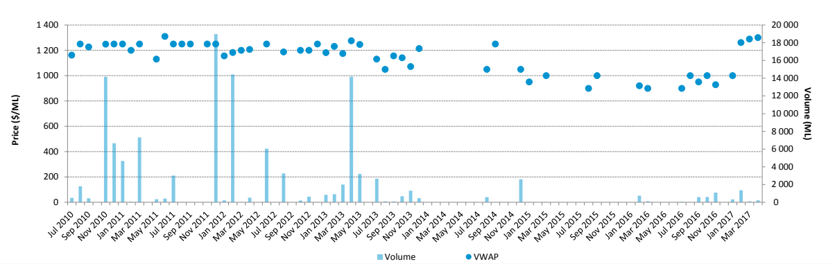
Entitlement market prices and volumes, Macquarie, general security, July 2010 to April 2017
