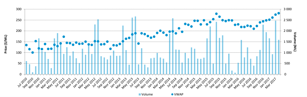
Entitlement market prices and volumes, Goulburn, low reliability, July 2010 to April 2017
