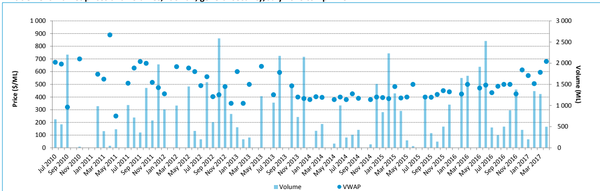
Entitlement market prices and volumes, Lachlan, general security, July 2010 to April 2017
