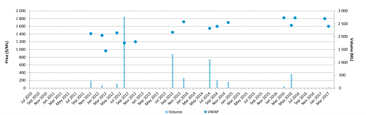
Entitlement market prices and volumes, Lower Darling, high security, July 2010 to April 2017
