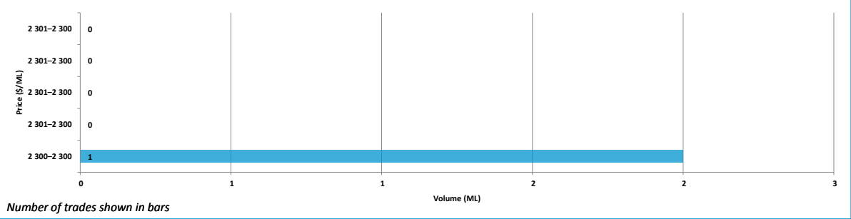
Entitlement market price range, Campaspe, high reliability, by volume month April 2017
