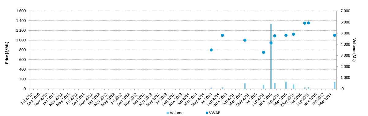
Entitlement market prices and volumes, Barwon–Darling, unregulated, July 2010 to April 2017
