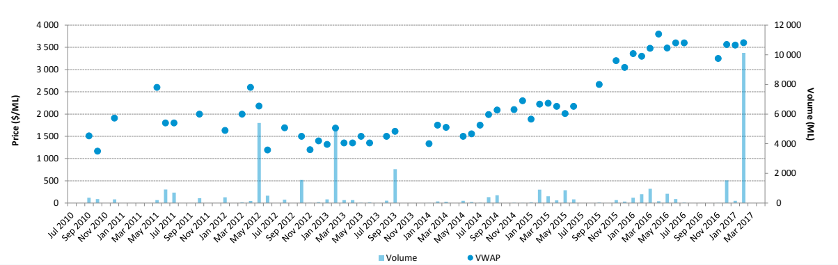
Entitlement market prices and volumes, Murrumbidgee, high security, July 2010 to April 2017
