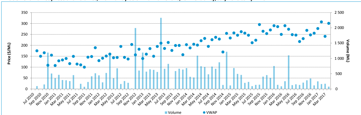
Entitlement market prices and volumes, Vic. Murray below Barmah Choke, low reliability, July 2010 to April 2017
