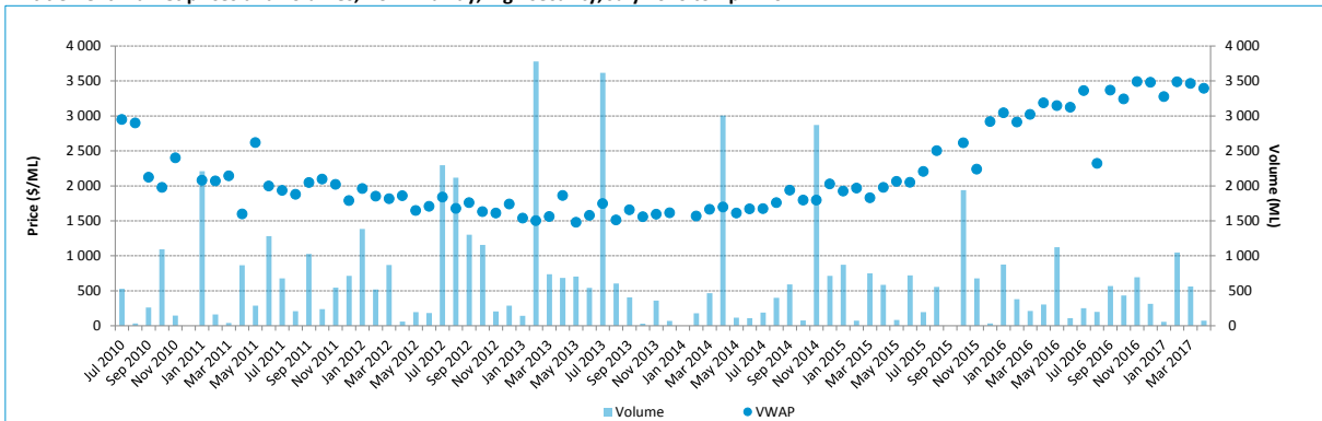
Entitlement market prices and volumes, NSW Murray, high security, July 2010 to April 2017
